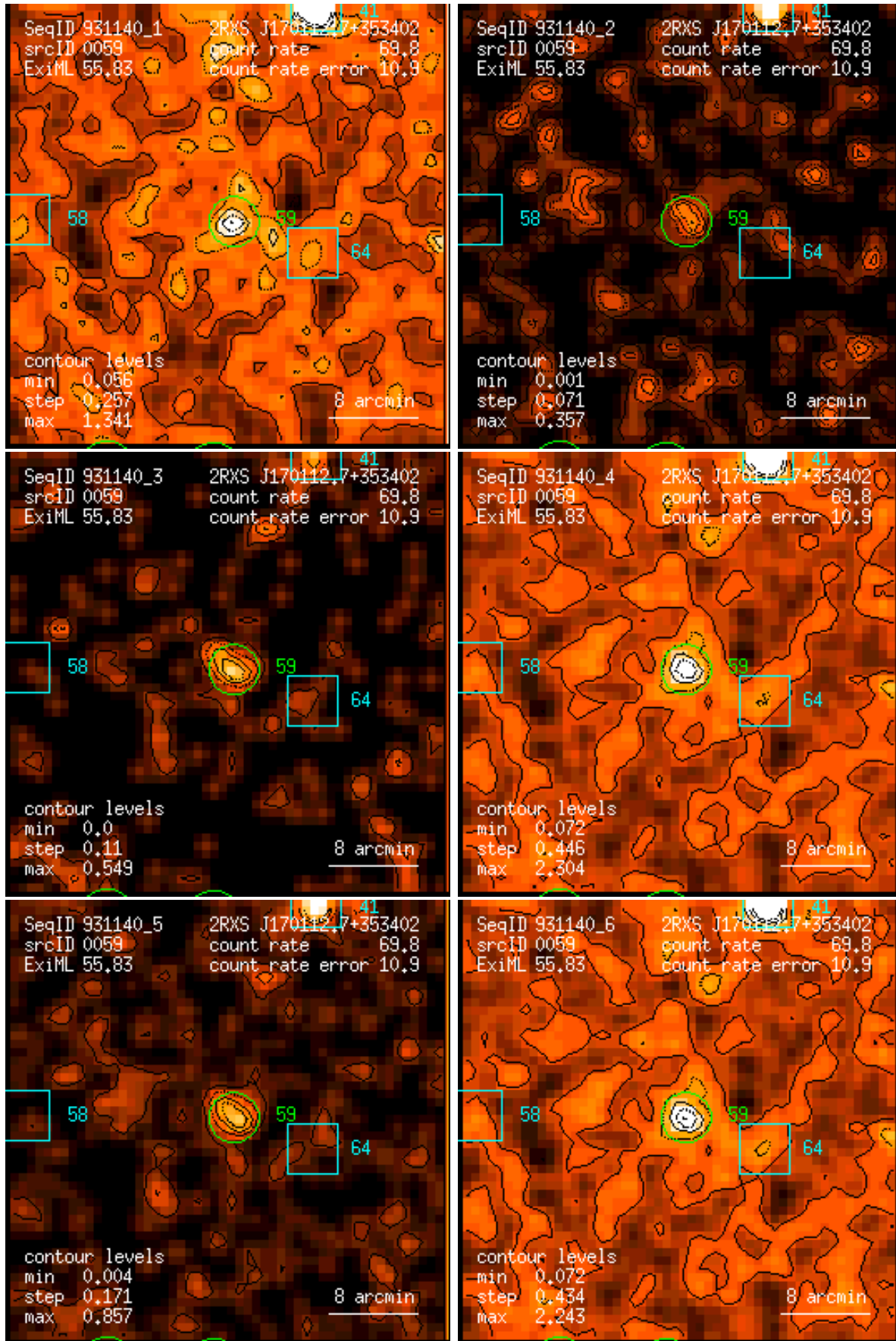
Figure 59: RASS 931140: detection 0059: band rate images, Gaussian filter: (1) PSPC channels 11 – 41, (2) 52 – 90, (3) 91 – 201, (4) 11 – 235, (5) 52 – 201, (6) 11 – 201. Broad band rates in counts/ks. Band rate contour levels in counts/ks/arcmin 2 .
