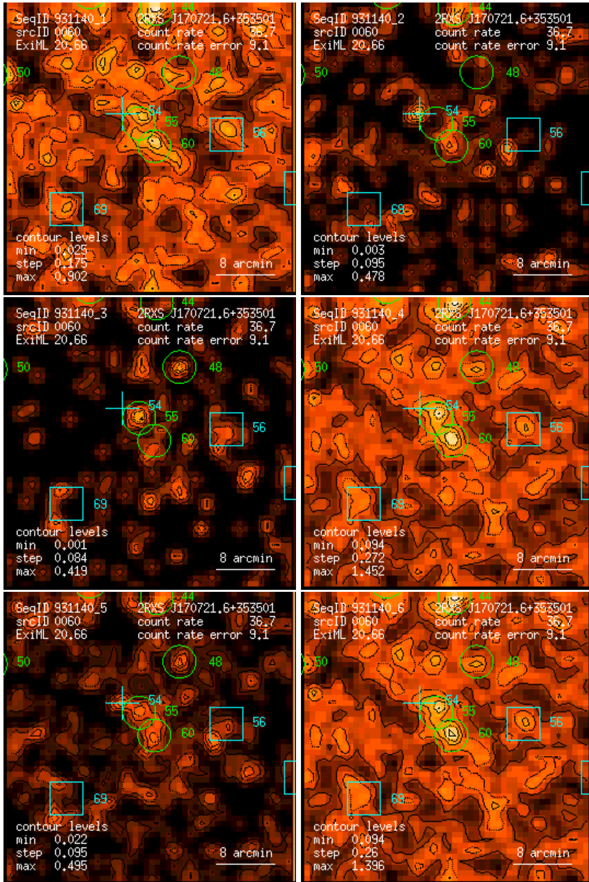
Figure 60: RASS 931140: detection 0060: band rate images, Gaussian filter: (1) PSPC channels 11 – 41, (2) 52 – 90, (3) 91 – 201, (4) 11 – 235, (5) 52 – 201, (6) 11 – 201. Broad band rates in counts/ks. Band rate contour levels in counts/ks/arcmin 2 .
