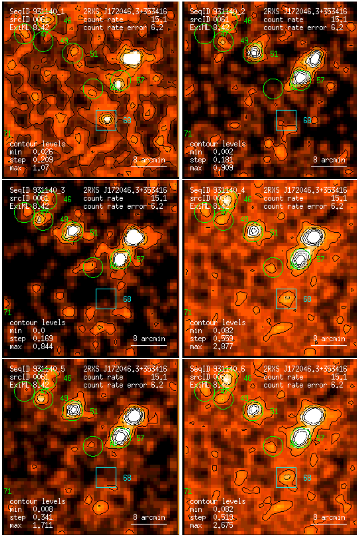
Figure 61: RASS 931140: detection 0061: band rate images, Gaussian filter: (1) PSPC channels 11 – 41, (2) 52 – 90, (3) 91 – 201, (4) 11 – 235, (5) 52 – 201, (6) 11 – 201. Broad band rates in counts/ks. Band rate contour levels in counts/ks/arcmin 2 .
