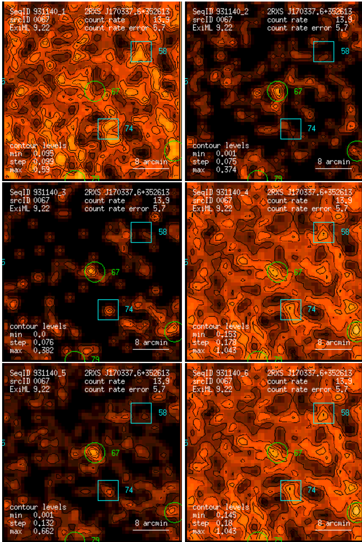
Figure 67: RASS 931140: detection 0067: band rate images, Gaussian filter: (1) PSPC channels 11 – 41, (2) 52 – 90, (3) 91 – 201, (4) 11 – 235, (5) 52 – 201, (6) 11 – 201. Broad band rates in counts/ks. Band rate contour levels in counts/ks/arcmin 2 .
