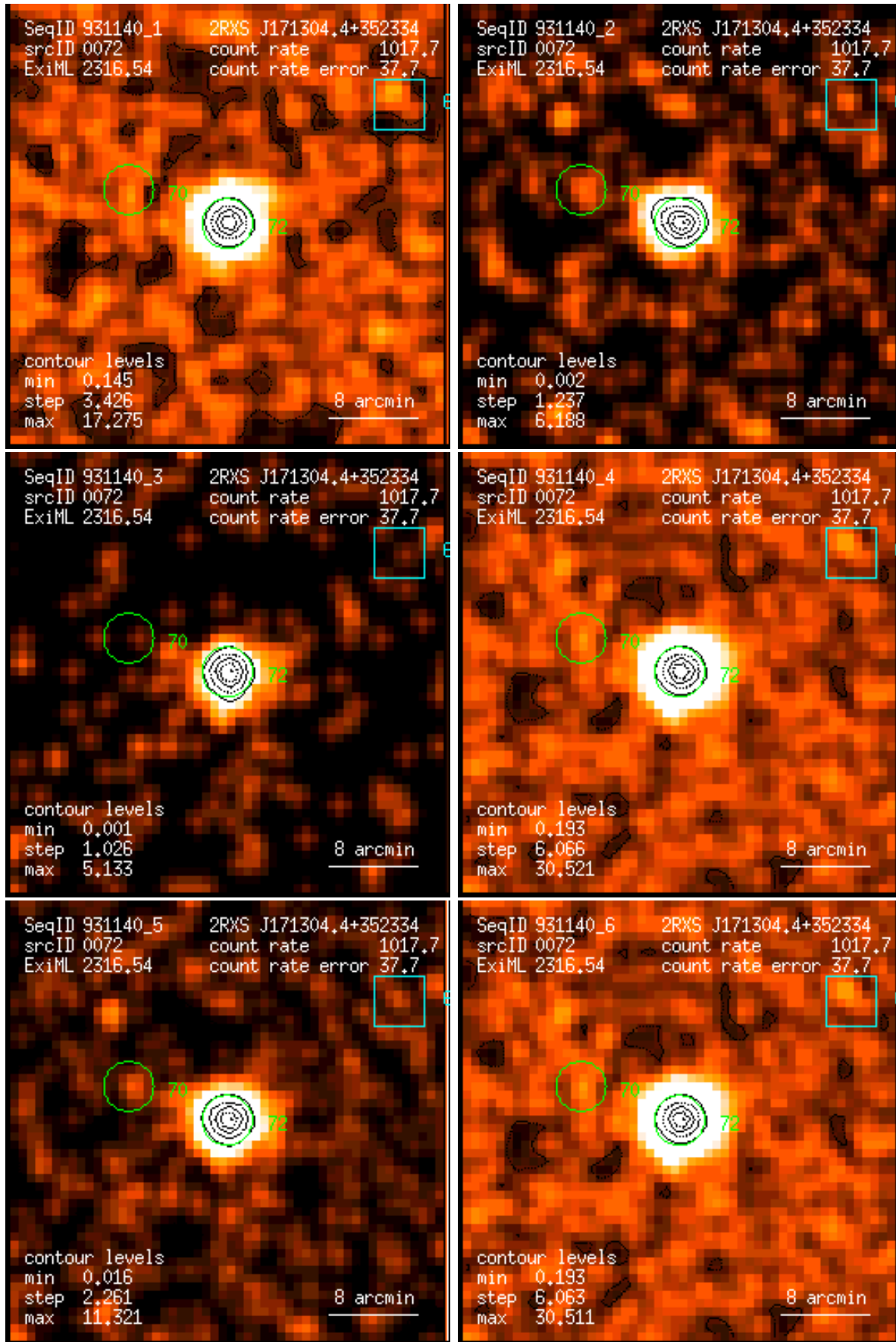
Figure 72: RASS 931140: detection 0072: band rate images, Gaussian filter: (1) PSPC channels 11 – 41, (2) 52 – 90, (3) 91 – 201, (4) 11 – 235, (5) 52 – 201, (6) 11 – 201. Broad band rates in counts/ks. Band rate contour levels in counts/ks/arcmin 2 .
