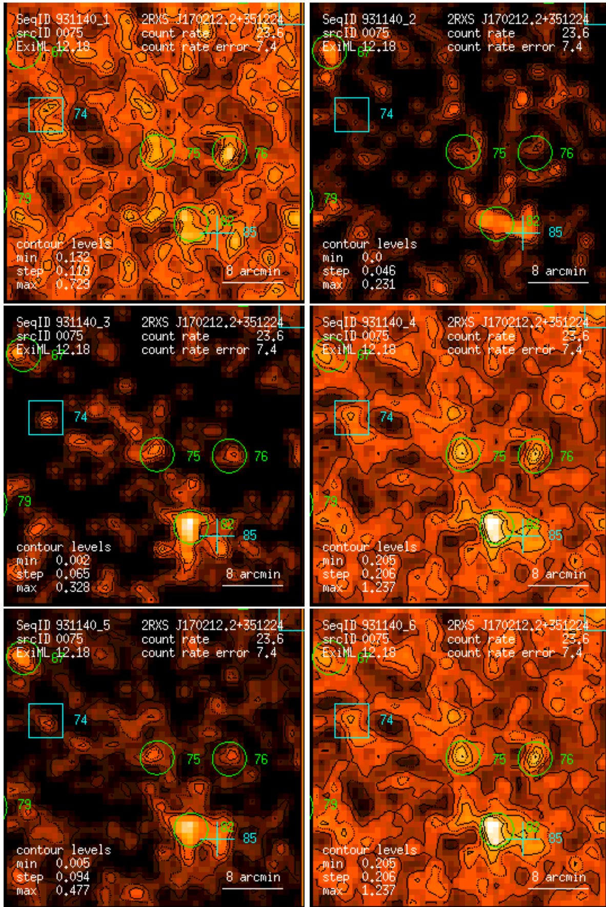
Figure 75: RASS 931140: detection 0075: band rate images, Gaussian filter: (1) PSPC channels 11 – 41, (2) 52 – 90, (3) 91 – 201, (4) 11 – 235, (5) 52 – 201, (6) 11 – 201. Broad band rates in counts/ks. Band rate contour levels in counts/ks/arcmin 2 .
