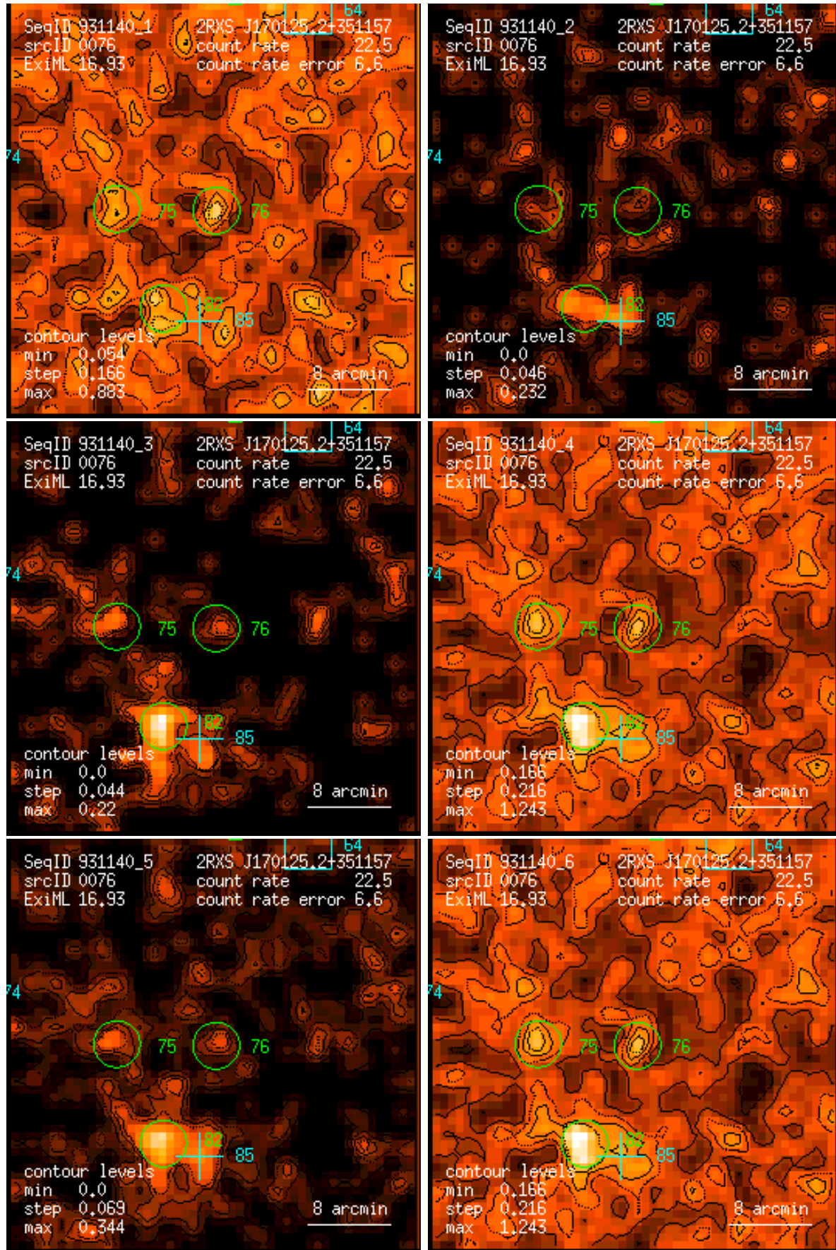
Figure 76: RASS 931140: detection 0076: band rate images, Gaussian filter: (1) PSPC channels 11 – 41, (2) 52 – 90, (3) 91 – 201, (4) 11 – 235, (5) 52 – 201, (6) 11 – 201. Broad band rates in counts/ks. Band rate contour levels in counts/ks/arcmin 2 .
