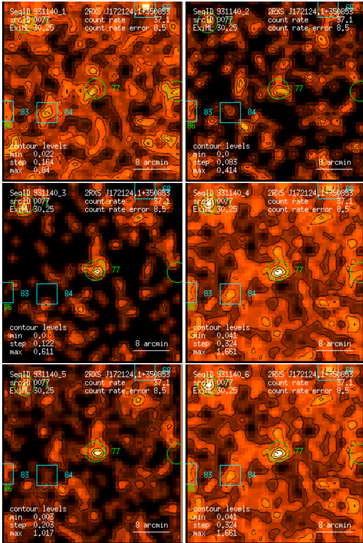
Figure 77: RASS 931140: detection 0077: band rate images, Gaussian filter: (1) PSPC channels 11 – 41, (2) 52 – 90, (3) 91 – 201, (4) 11 – 235, (5) 52 – 201, (6) 11 – 201. Broad band rates in counts/ks. Band rate contour levels in counts/ks/arcmin 2 .
