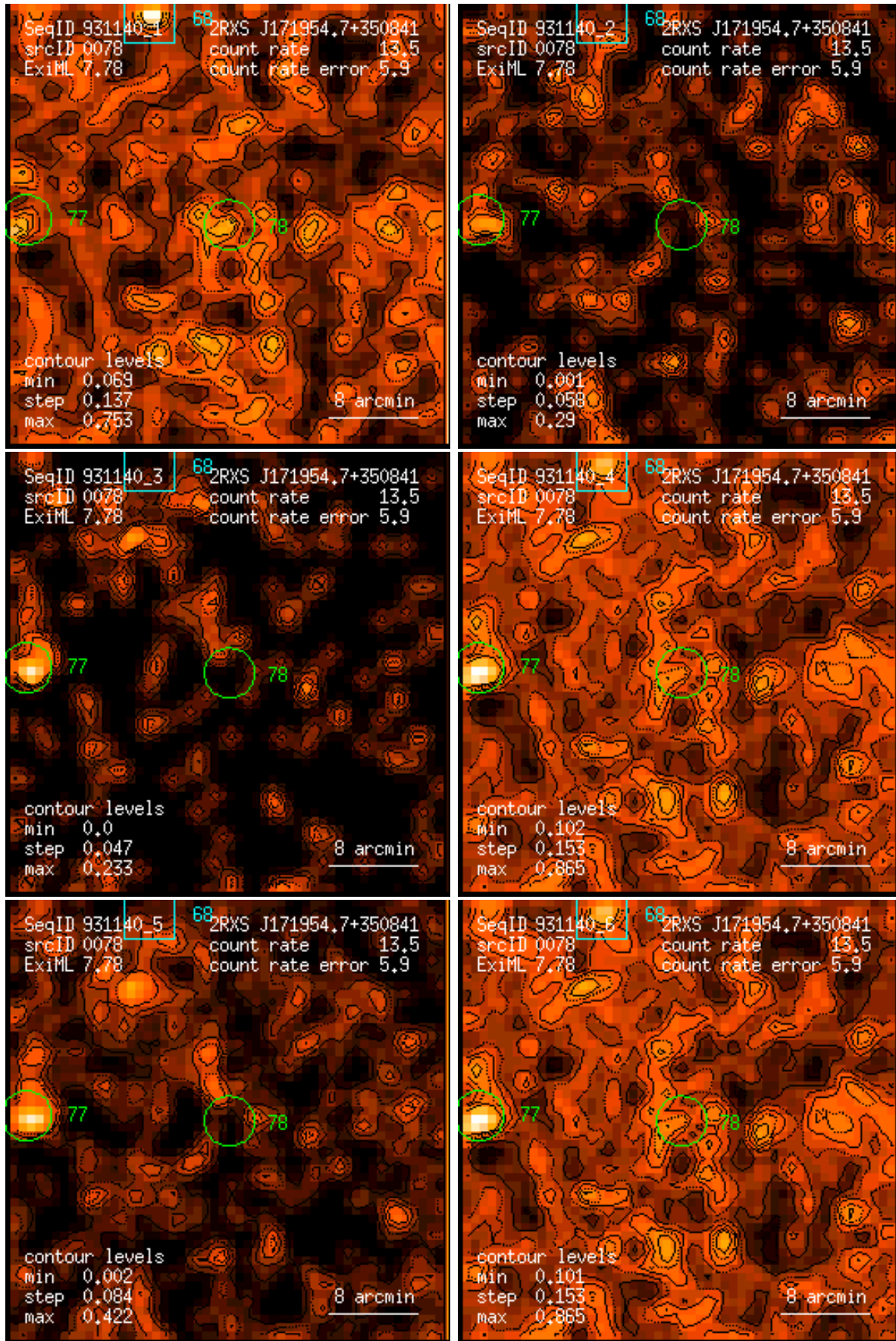
Figure 78: RASS 931140: detection 0078: band rate images, Gaussian filter: (1) PSPC channels 11 – 41, (2) 52 – 90, (3) 91 – 201, (4) 11 – 235, (5) 52 – 201, (6) 11 – 201. Broad band rates in counts/ks. Band rate contour levels in counts/ks/arcmin 2 .
