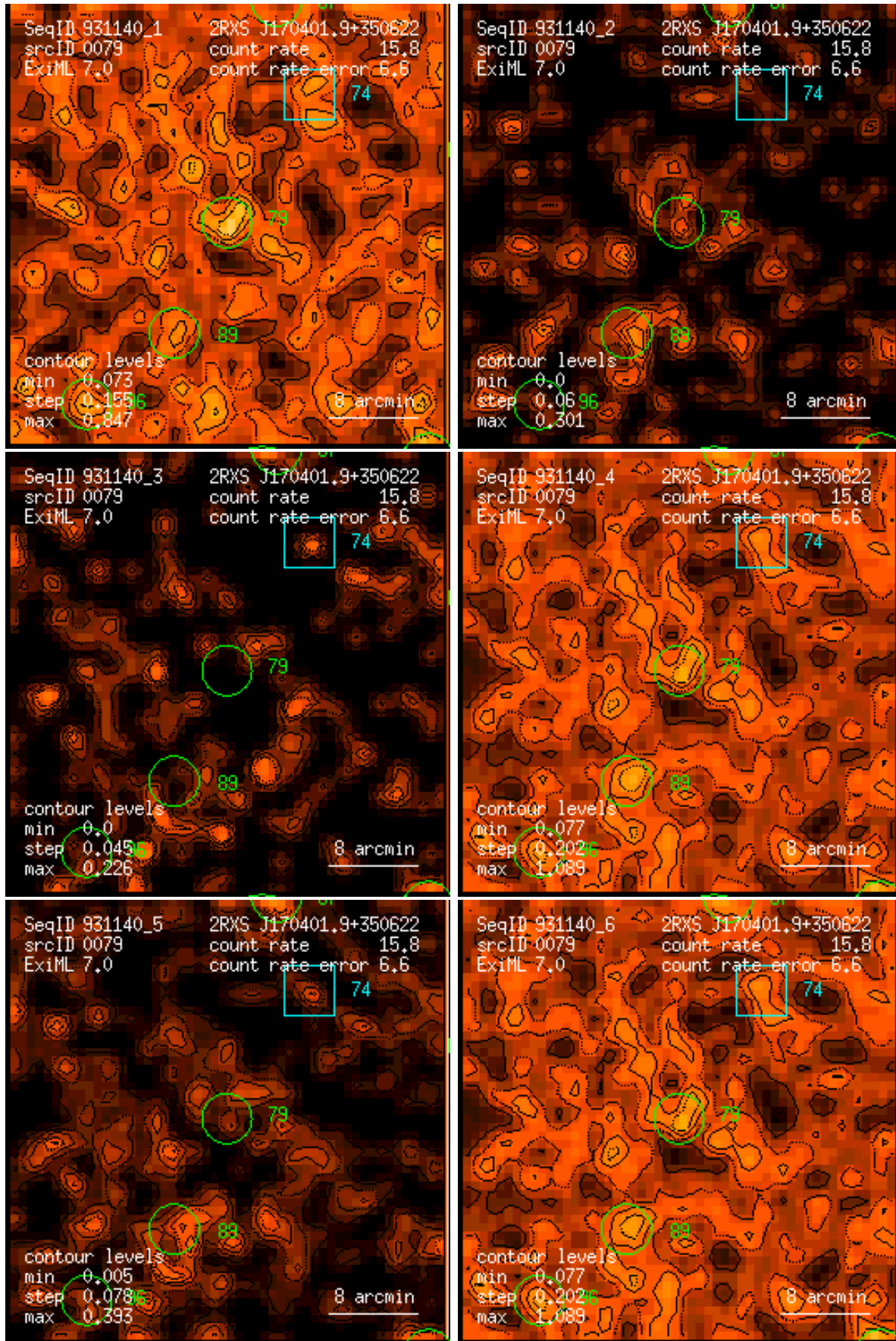
Figure 79: RASS 931140: detection 0079: band rate images, Gaussian filter: (1) PSPC channels 11 – 41, (2) 52 – 90, (3) 91 – 201, (4) 11 – 235, (5) 52 – 201, (6) 11 – 201. Broad band rates in counts/ks. Band rate contour levels in counts/ks/arcmin 2 .
