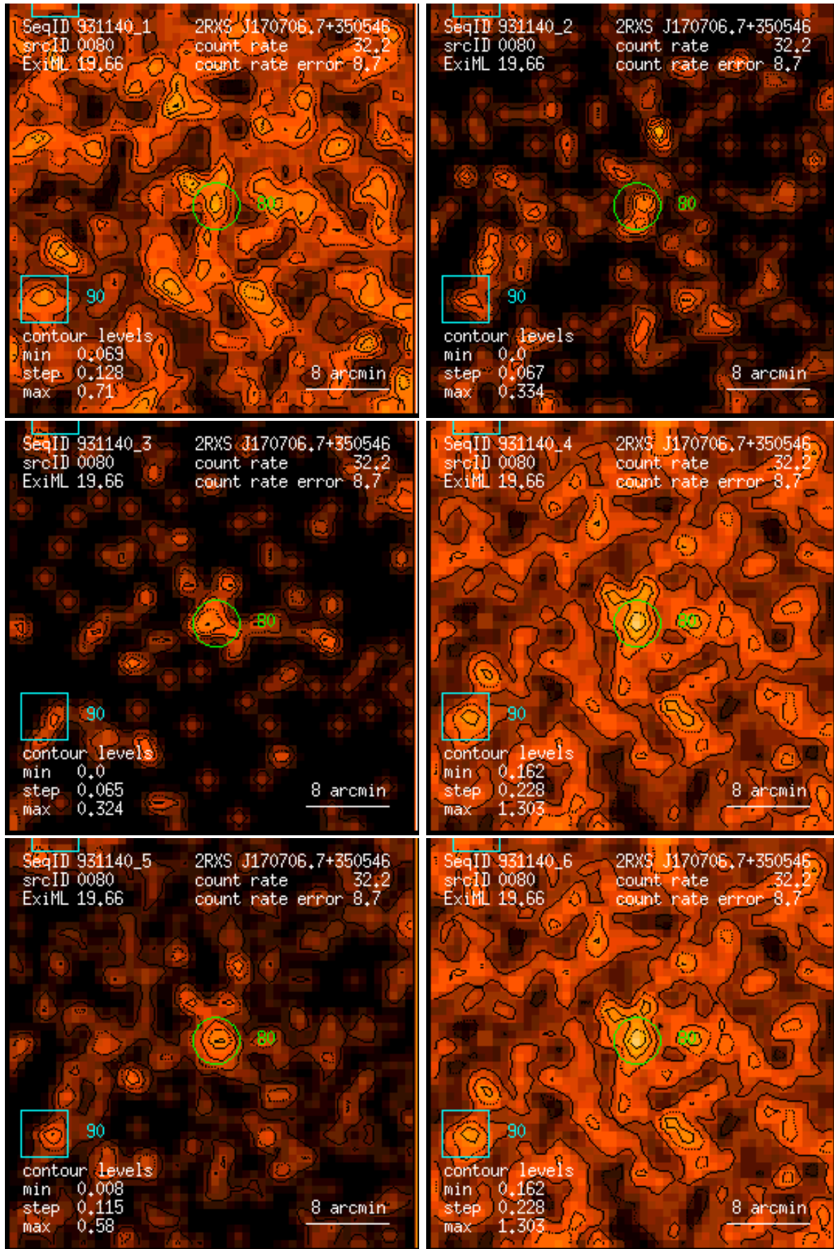
Figure 80: RASS 931140: detection 0080: band rate images, Gaussian filter: (1) PSPC channels 11 – 41, (2) 52 – 90, (3) 91 – 201, (4) 11 – 235, (5) 52 – 201, (6) 11 – 201. Broad band rates in counts/ks. Band rate contour levels in counts/ks/arcmin 2 .
