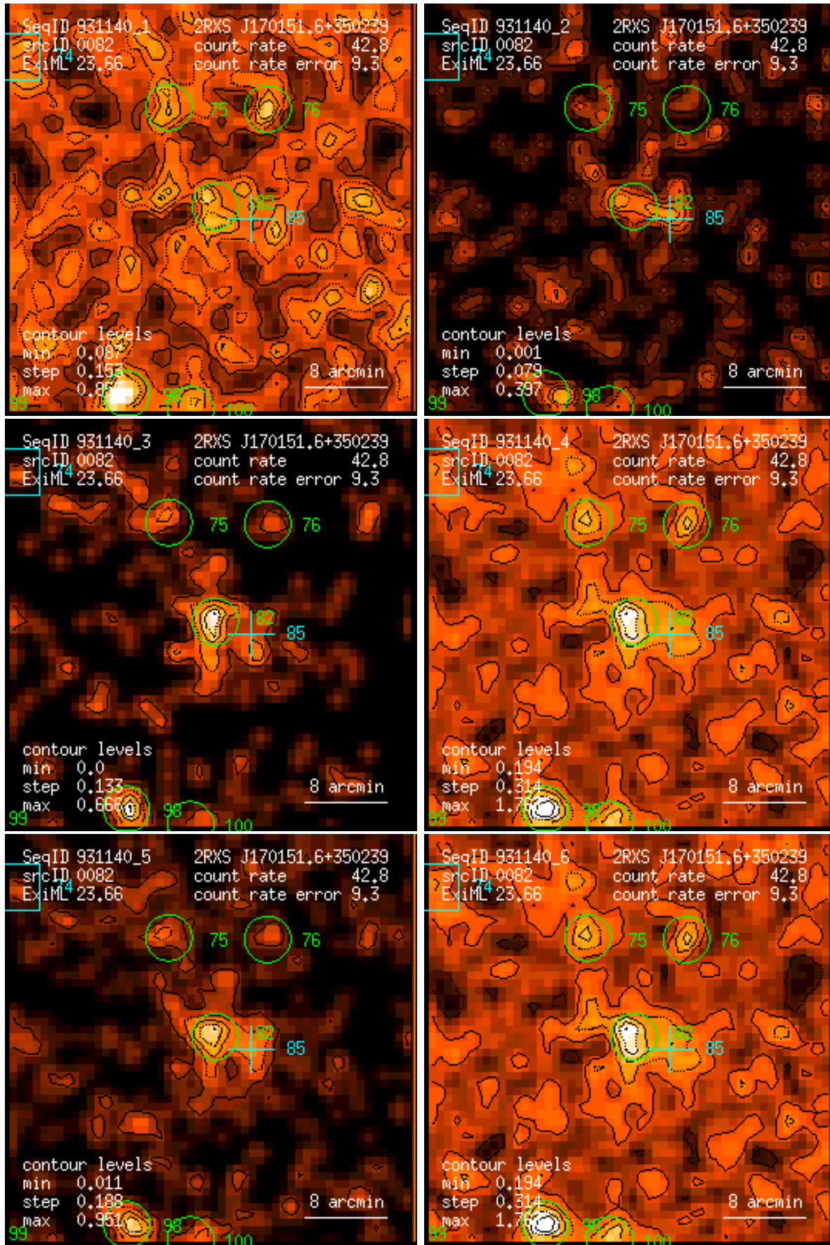
Figure 82: RASS 931140: detection 0082: band rate images, Gaussian filter: (1) PSPC channels 11 – 41, (2) 52 – 90, (3) 91 – 201, (4) 11 – 235, (5) 52 – 201, (6) 11 – 201. Broad band rates in counts/ks. Band rate contour levels in counts/ks/arcmin 2 .
