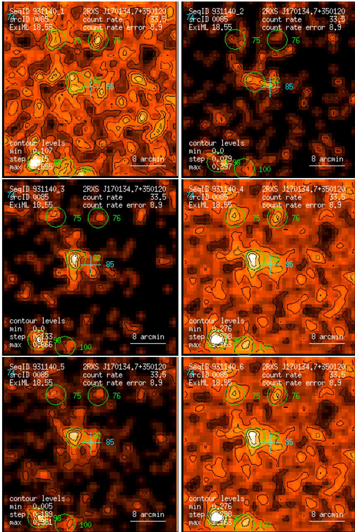
Figure 85: RASS 931140: detection 0085: band rate images, Gaussian filter: (1) PSPC channels 11 – 41, (2) 52 – 90, (3) 91 – 201, (4) 11 – 235, (5) 52 – 201, (6) 11 – 201. Broad band rates in counts/ks. Band rate contour levels in counts/ks/arcmin 2 .
