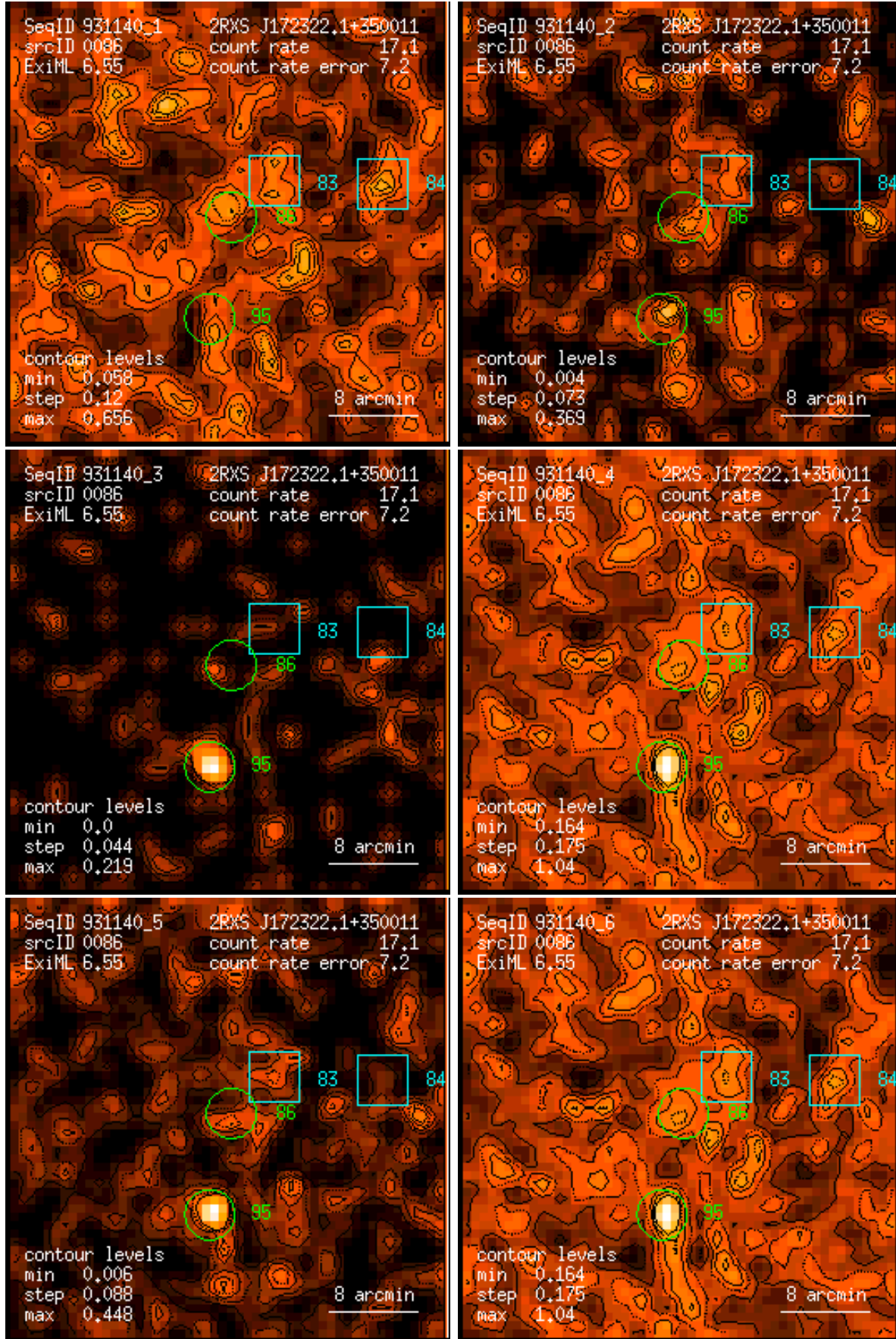
Figure 86: RASS 931140: detection 0086: band rate images, Gaussian filter: (1) PSPC channels 11 – 41, (2) 52 – 90, (3) 91 – 201, (4) 11 – 235, (5) 52 – 201, (6) 11 – 201. Broad band rates in counts/ks. Band rate contour levels in counts/ks/arcmin 2 .
