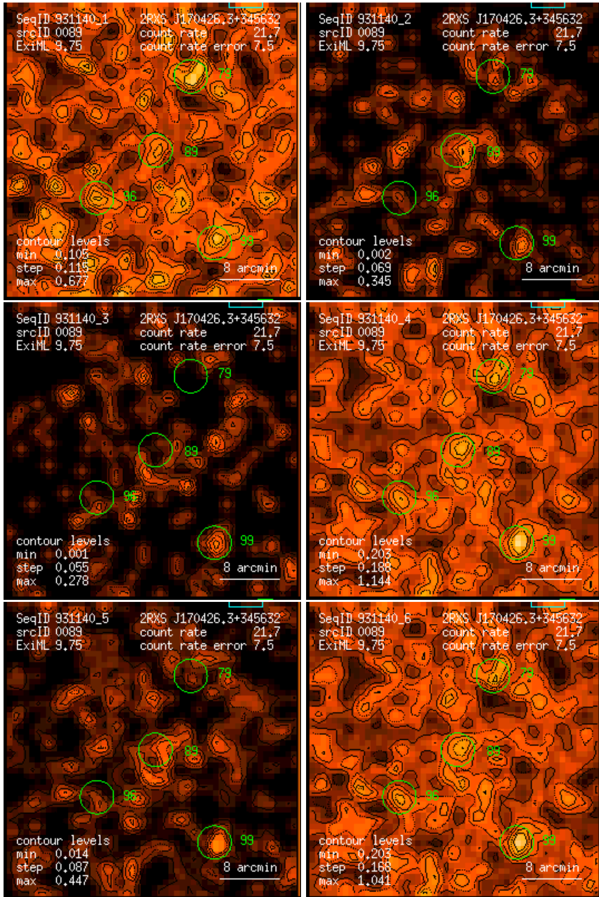
Figure 89: RASS 931140: detection 0089: band rate images, Gaussian filter: (1) PSPC channels 11 – 41, (2) 52 – 90, (3) 91 – 201, (4) 11 – 235, (5) 52 – 201, (6) 11 – 201. Broad band rates in counts/ks. Band rate contour levels in counts/ks/arcmin 2 .
