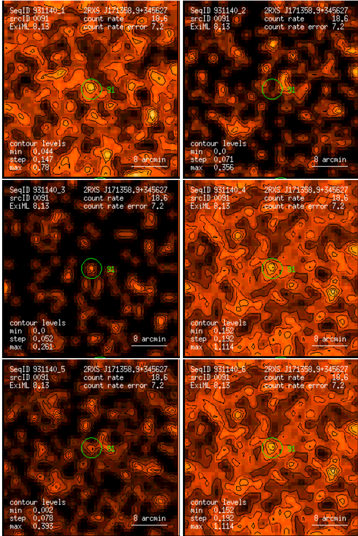
Figure 91: RASS 931140: detection 0091: band rate images, Gaussian filter: (1) PSPC channels 11 – 41, (2) 52 – 90, (3) 91 – 201, (4) 11 – 235, (5) 52 – 201, (6) 11 – 201. Broad band rates in counts/ks. Band rate contour levels in counts/ks/arcmin 2 .
