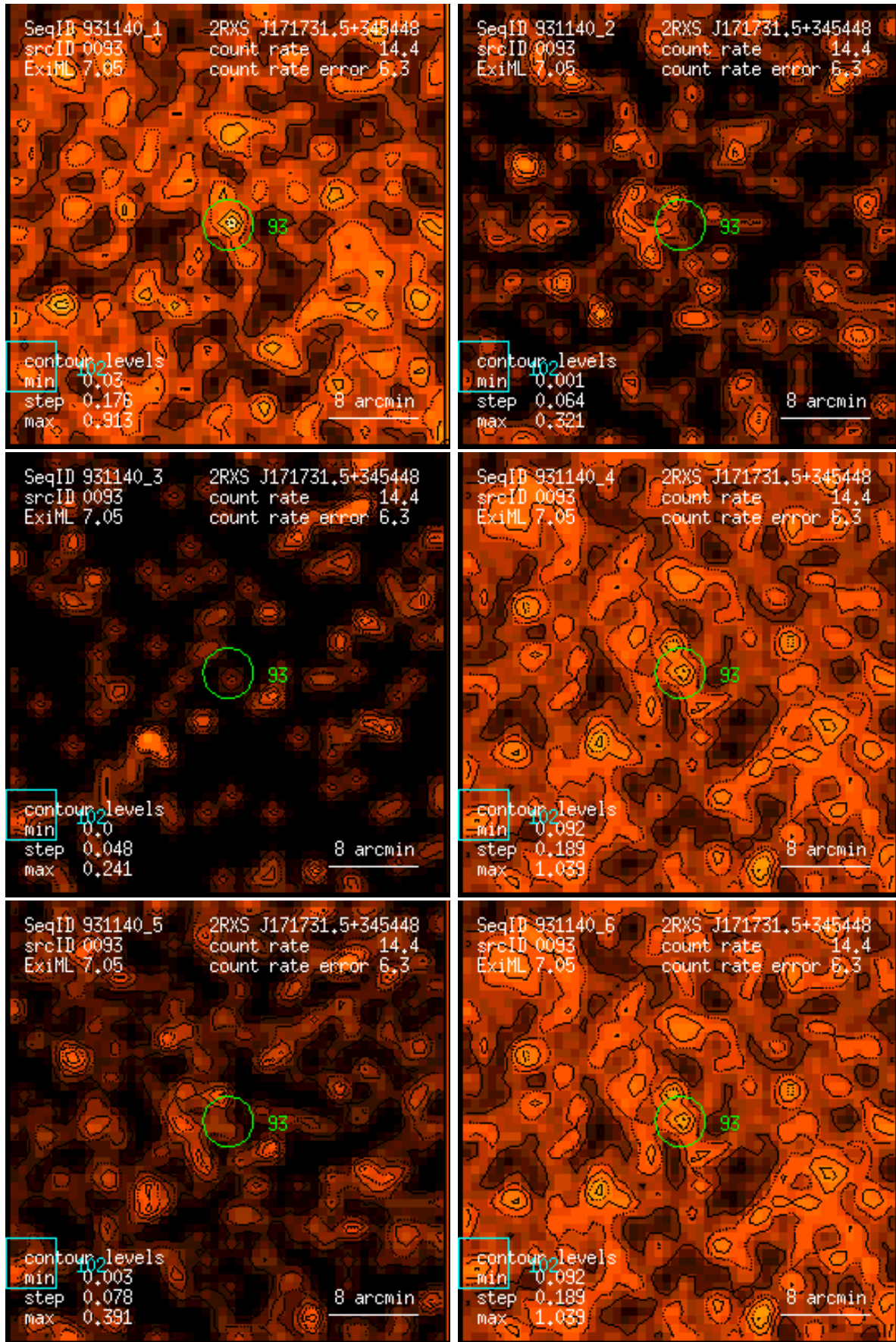
Figure 93: RASS 931140: detection 0093: band rate images, Gaussian filter: (1) PSPC channels 11 – 41, (2) 52 – 90, (3) 91 – 201, (4) 11 – 235, (5) 52 – 201, (6) 11 – 201. Broad band rates in counts/ks. Band rate contour levels in counts/ks/arcmin 2 .
