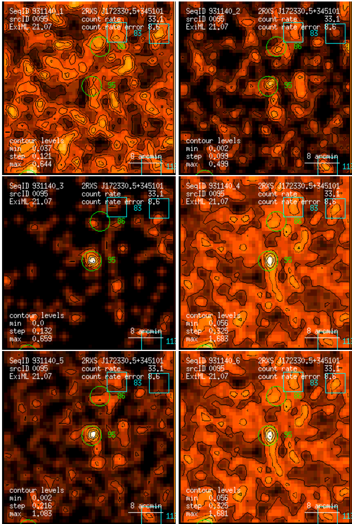
Figure 95: RASS 931140: detection 0095: band rate images, Gaussian filter: (1) PSPC channels 11 – 41, (2) 52 – 90, (3) 91 – 201, (4) 11 – 235, (5) 52 – 201, (6) 11 – 201. Broad band rates in counts/ks. Band rate contour levels in counts/ks/arcmin 2 .
