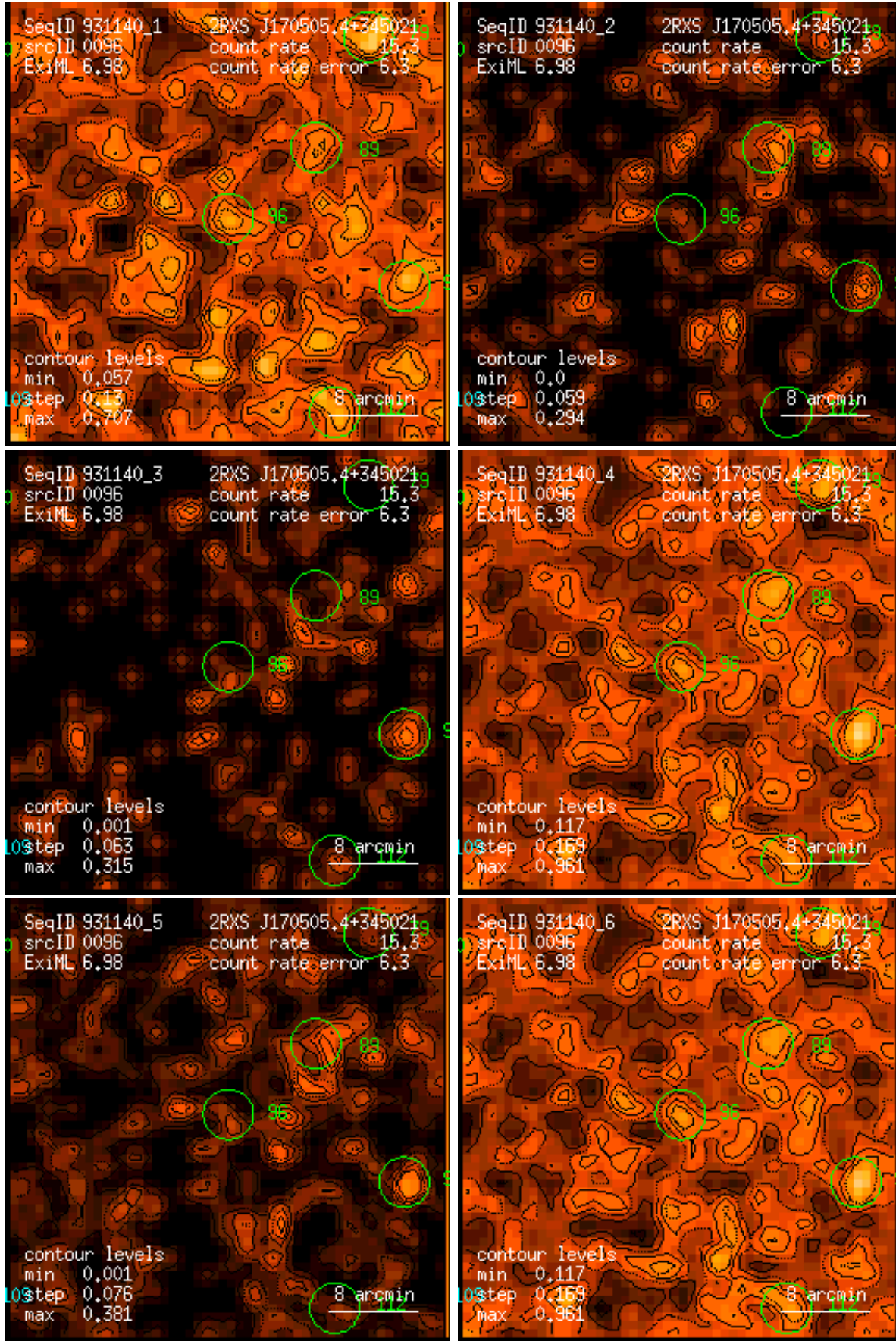
Figure 96: RASS 931140: detection 0096: band rate images, Gaussian filter: (1) PSPC channels 11 – 41, (2) 52 – 90, (3) 91 – 201, (4) 11 – 235, (5) 52 – 201, (6) 11 – 201. Broad band rates in counts/ks. Band rate contour levels in counts/ks/arcmin 2 .
