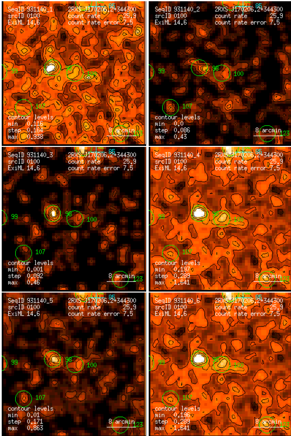
Figure 100: RASS 931140: detection 0100: band rate images, Gaussian filter: (1) PSPC channels 11 – 41, (2) 52 – 90, (3) 91 – 201, (4) 11 – 235, (5) 52 – 201, (6) 11 – 201. Broad band rates in counts/ks. Band rate contour levels in counts/ks/arcmin 2 .
