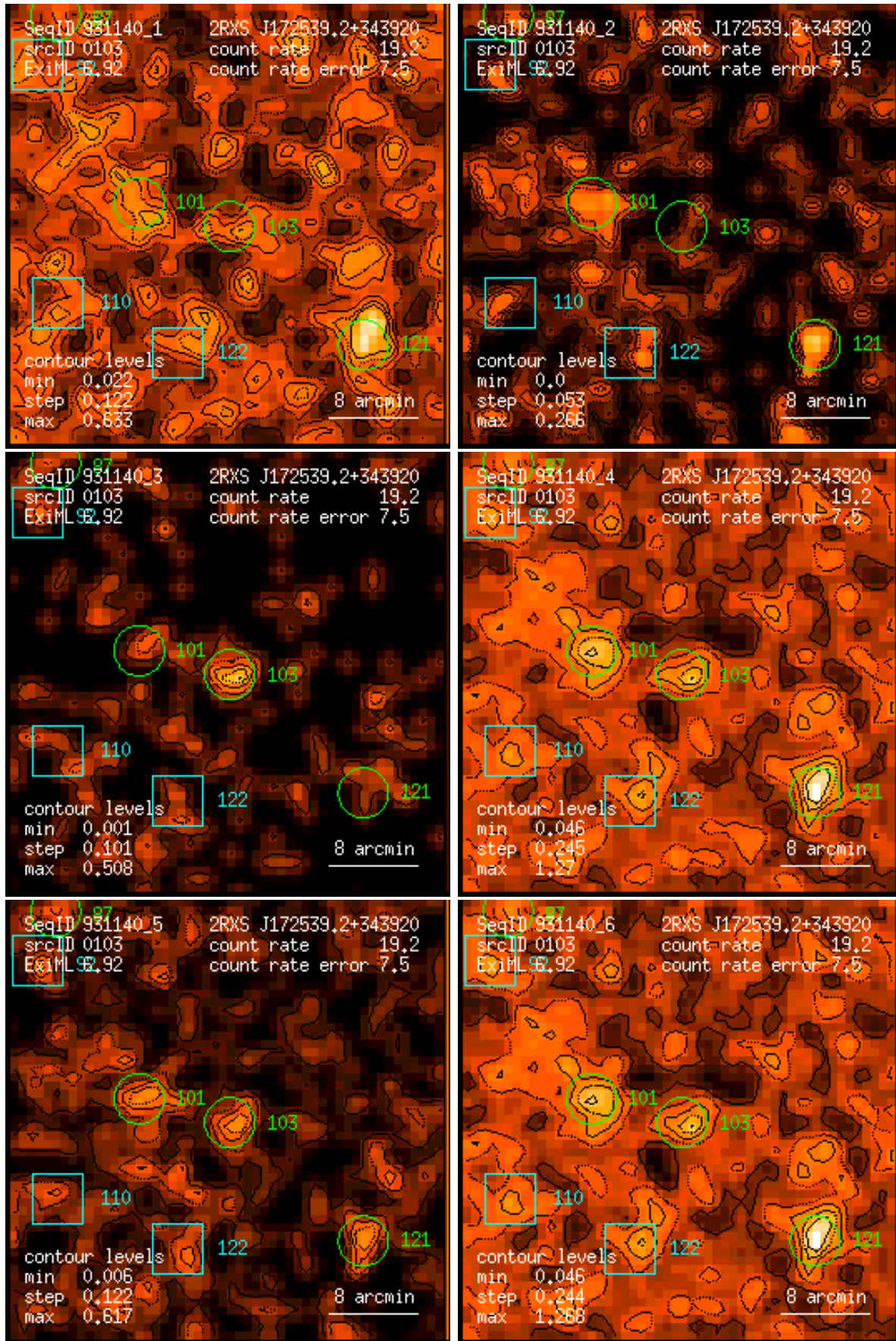
Figure 103: RASS 931140: detection 0103: band rate images, Gaussian filter: (1) PSPC channels 11 – 41, (2) 52 – 90, (3) 91 – 201, (4) 11 – 235, (5) 52 – 201, (6) 11 – 201. Broad band rates in counts/ks. Band rate contour levels in counts/ks/arcmin 2 .
