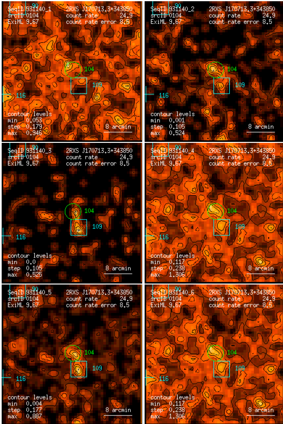
Figure 104: RASS 931140: detection 0104: band rate images, Gaussian filter: (1) PSPC channels 11 – 41, (2) 52 – 90, (3) 91 – 201, (4) 11 – 235, (5) 52 – 201, (6) 11 – 201. Broad band rates in counts/ks. Band rate contour levels in counts/ks/arcmin 2 .
