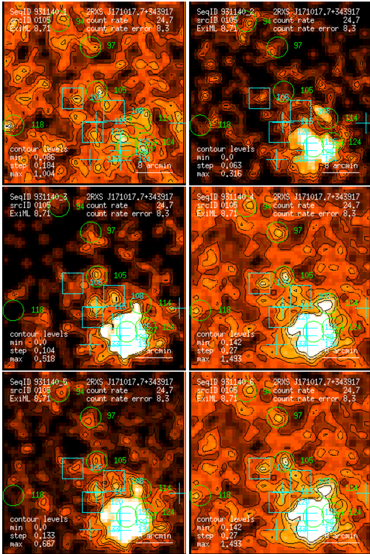
Figure 105: RASS 931140: detection 0105: band rate images, Gaussian filter: (1) PSPC channels 11 – 41, (2) 52 – 90, (3) 91 – 201, (4) 11 – 235, (5) 52 – 201, (6) 11 – 201. Broad band rates in counts/ks. Band rate contour levels in counts/ks/arcmin 2 .
