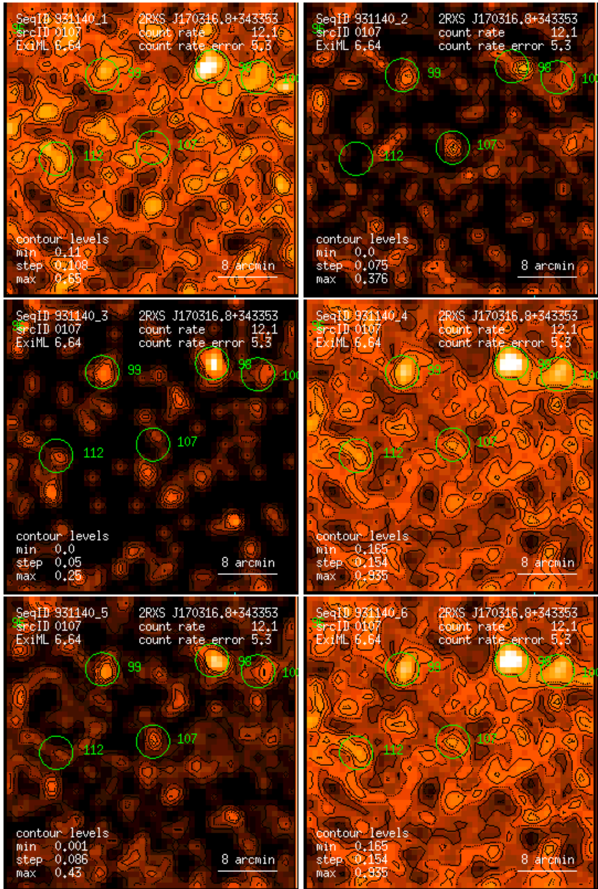
Figure 107: RASS 931140: detection 0107: band rate images, Gaussian filter: (1) PSPC channels 11 – 41, (2) 52 – 90, (3) 91 – 201, (4) 11 – 235, (5) 52 – 201, (6) 11 – 201. Broad band rates in counts/ks. Band rate contour levels in counts/ks/arcmin 2 .
