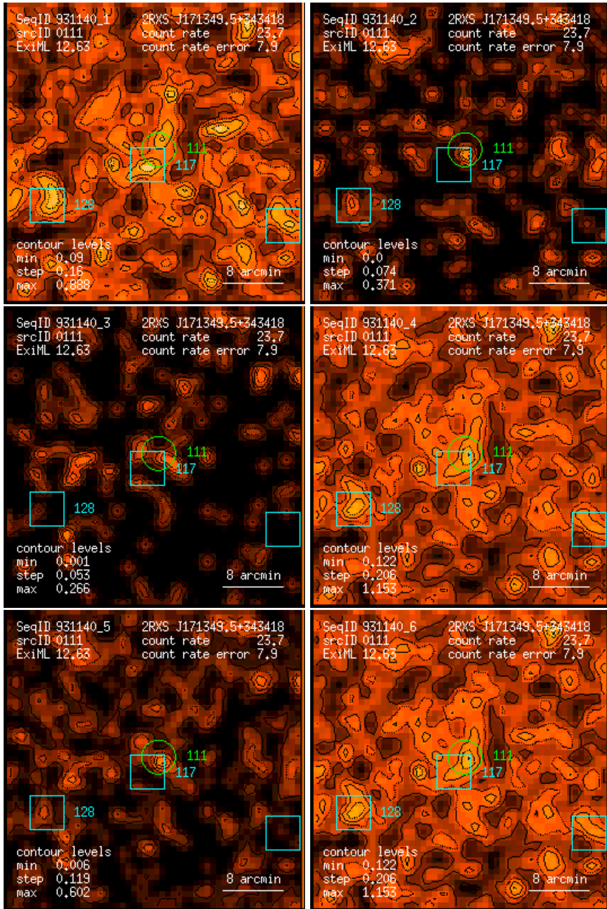
Figure 111: RASS 931140: detection 0111: band rate images, Gaussian filter: (1) PSPC channels 11 – 41, (2) 52 – 90, (3) 91 – 201, (4) 11 – 235, (5) 52 – 201, (6) 11 – 201. Broad band rates in counts/ks. Band rate contour levels in counts/ks/arcmin 2 .
