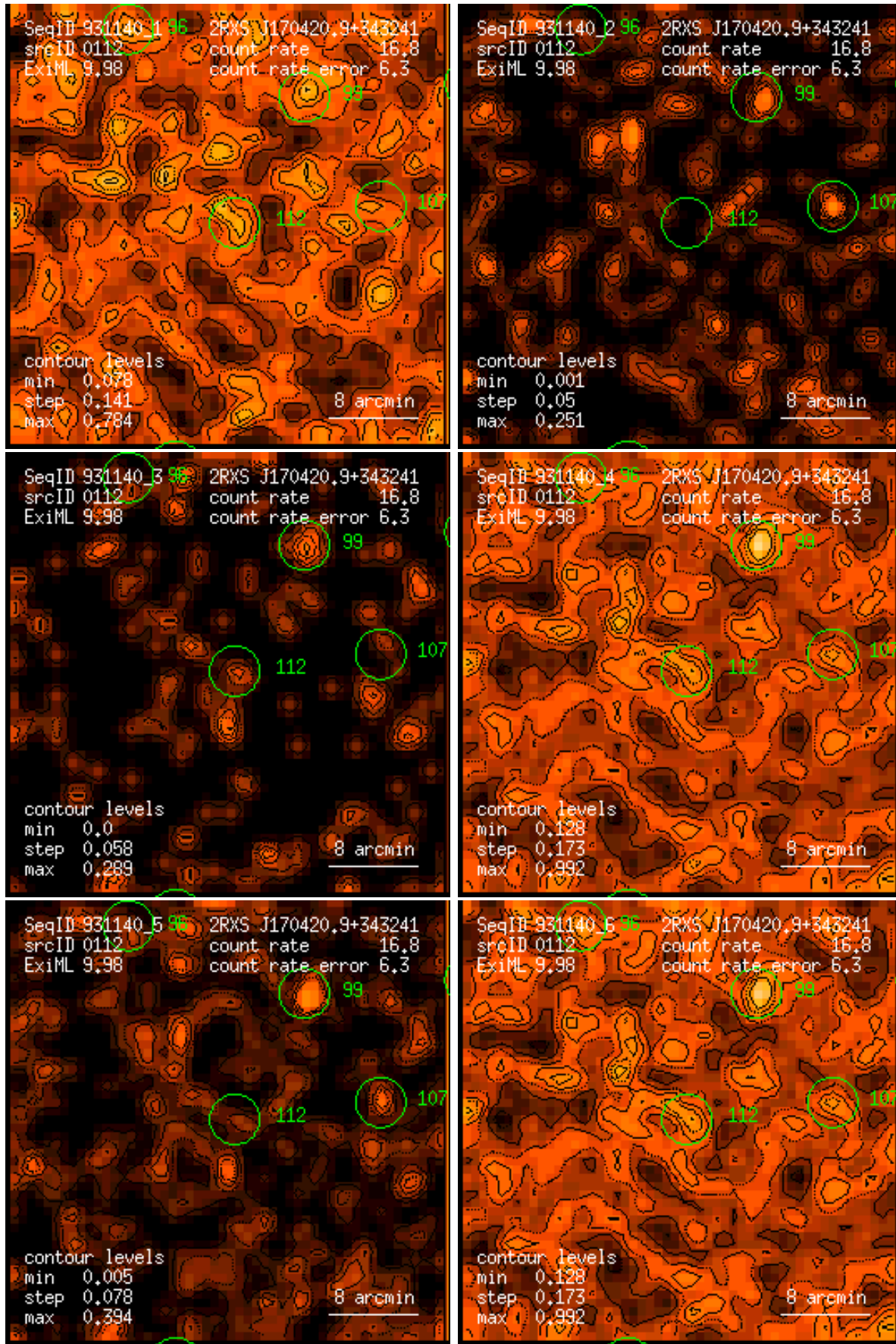
Figure 112: RASS 931140: detection 0112: band rate images, Gaussian filter: (1) PSPC channels 11 – 41, (2) 52 – 90, (3) 91 – 201, (4) 11 – 235, (5) 52 – 201, (6) 11 – 201. Broad band rates in counts/ks. Band rate contour levels in counts/ks/arcmin 2 .
