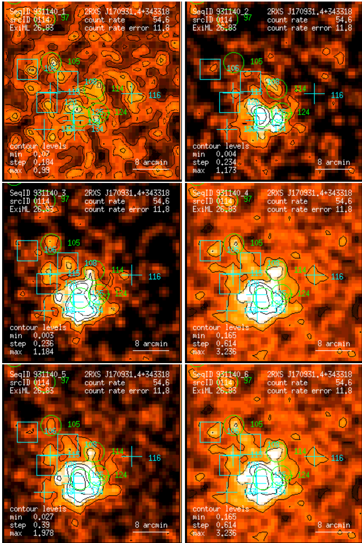
Figure 114: RASS 931140: detection 0114: band rate images, Gaussian filter: (1) PSPC channels 11 – 41, (2) 52 – 90, (3) 91 – 201, (4) 11 – 235, (5) 52 – 201, (6) 11 – 201. Broad band rates in counts/ks. Band rate contour levels in counts/ks/arcmin 2 .
