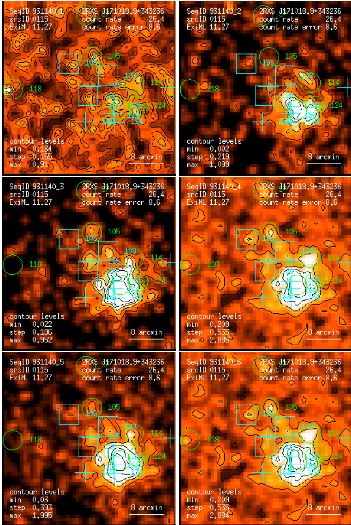
Figure 115: RASS 931140: detection 0115: band rate images, Gaussian filter: (1) PSPC channels 11 – 41, (2) 52 – 90, (3) 91 – 201, (4) 11 – 235, (5) 52 – 201, (6) 11 – 201. Broad band rates in counts/ks. Band rate contour levels in counts/ks/arcmin 2 .
