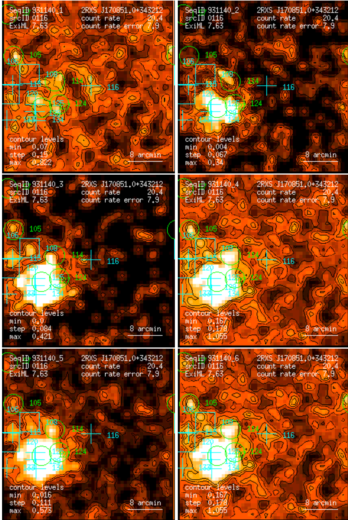
Figure 116: RASS 931140: detection 0116: band rate images, Gaussian filter: (1) PSPC channels 11 – 41, (2) 52 – 90, (3) 91 – 201, (4) 11 – 235, (5) 52 – 201, (6) 11 – 201. Broad band rates in counts/ks. Band rate contour levels in counts/ks/arcmin 2 .
