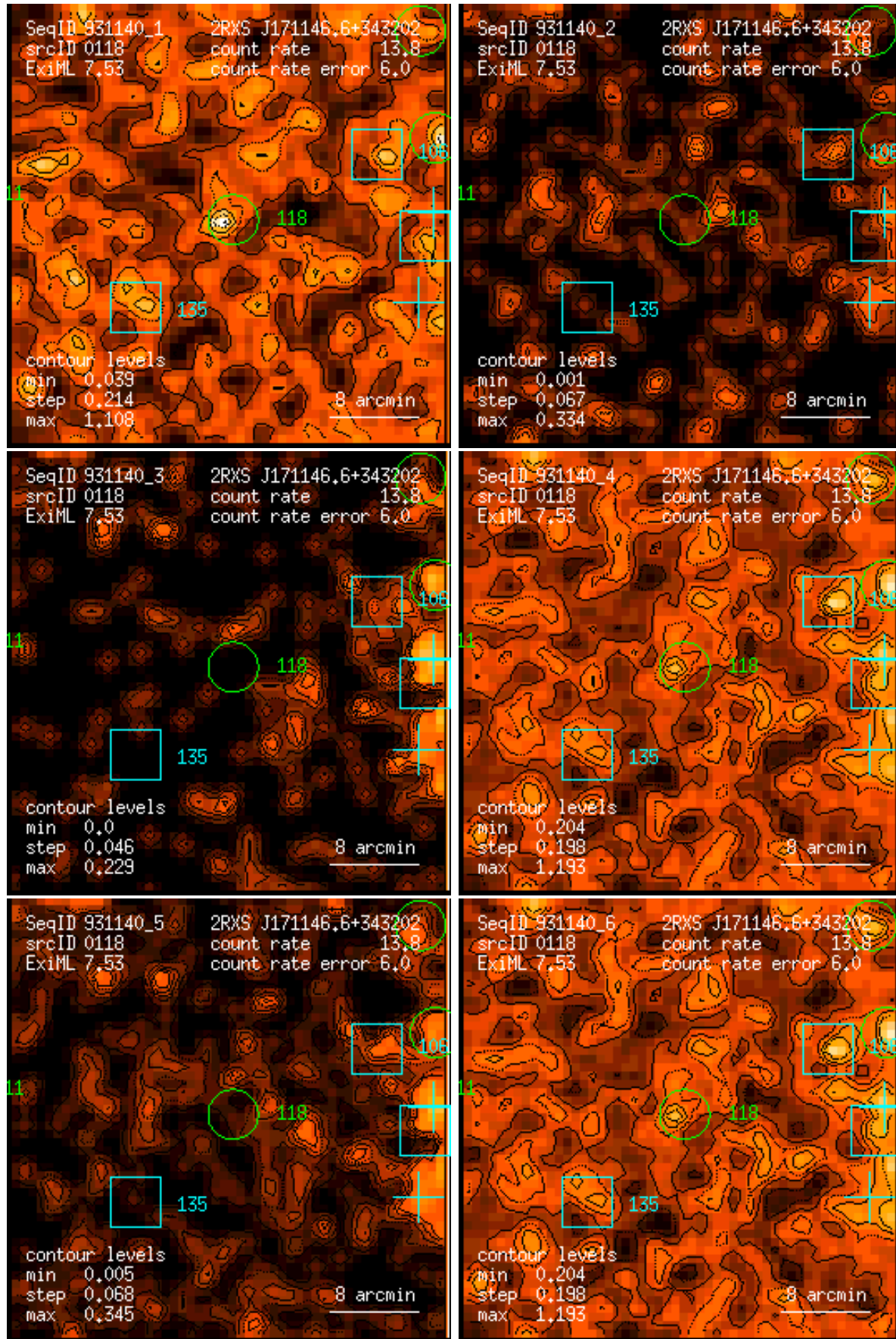
Figure 118: RASS 931140: detection 0118: band rate images, Gaussian filter: (1) PSPC channels 11 – 41, (2) 52 – 90, (3) 91 – 201, (4) 11 – 235, (5) 52 – 201, (6) 11 – 201. Broad band rates in counts/ks. Band rate contour levels in counts/ks/arcmin 2 .
