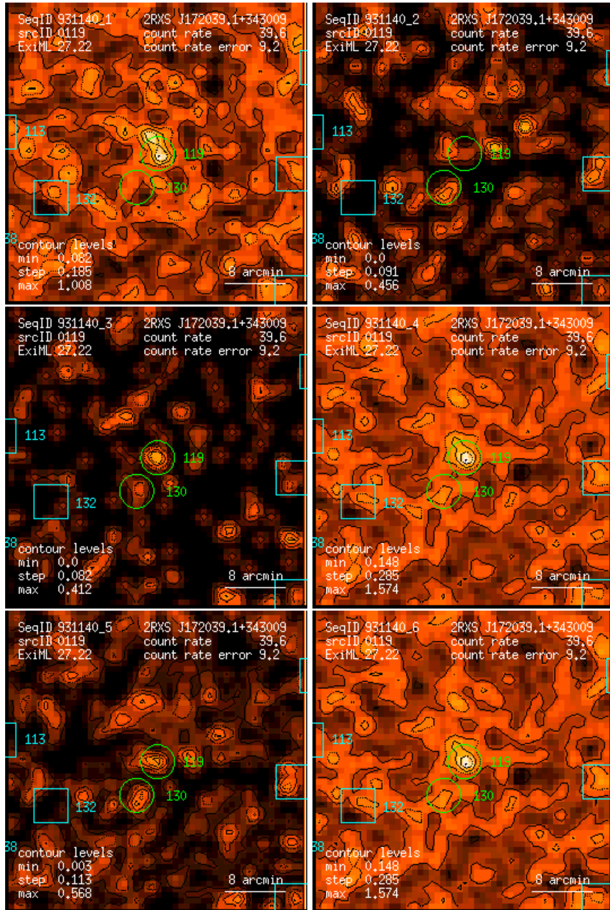
Figure 119: RASS 931140: detection 0119: band rate images, Gaussian filter: (1) PSPC channels 11 – 41, (2) 52 – 90, (3) 91 – 201, (4) 11 – 235, (5) 52 – 201, (6) 11 – 201. Broad band rates in counts/ks. Band rate contour levels in counts/ks/arcmin 2 .
