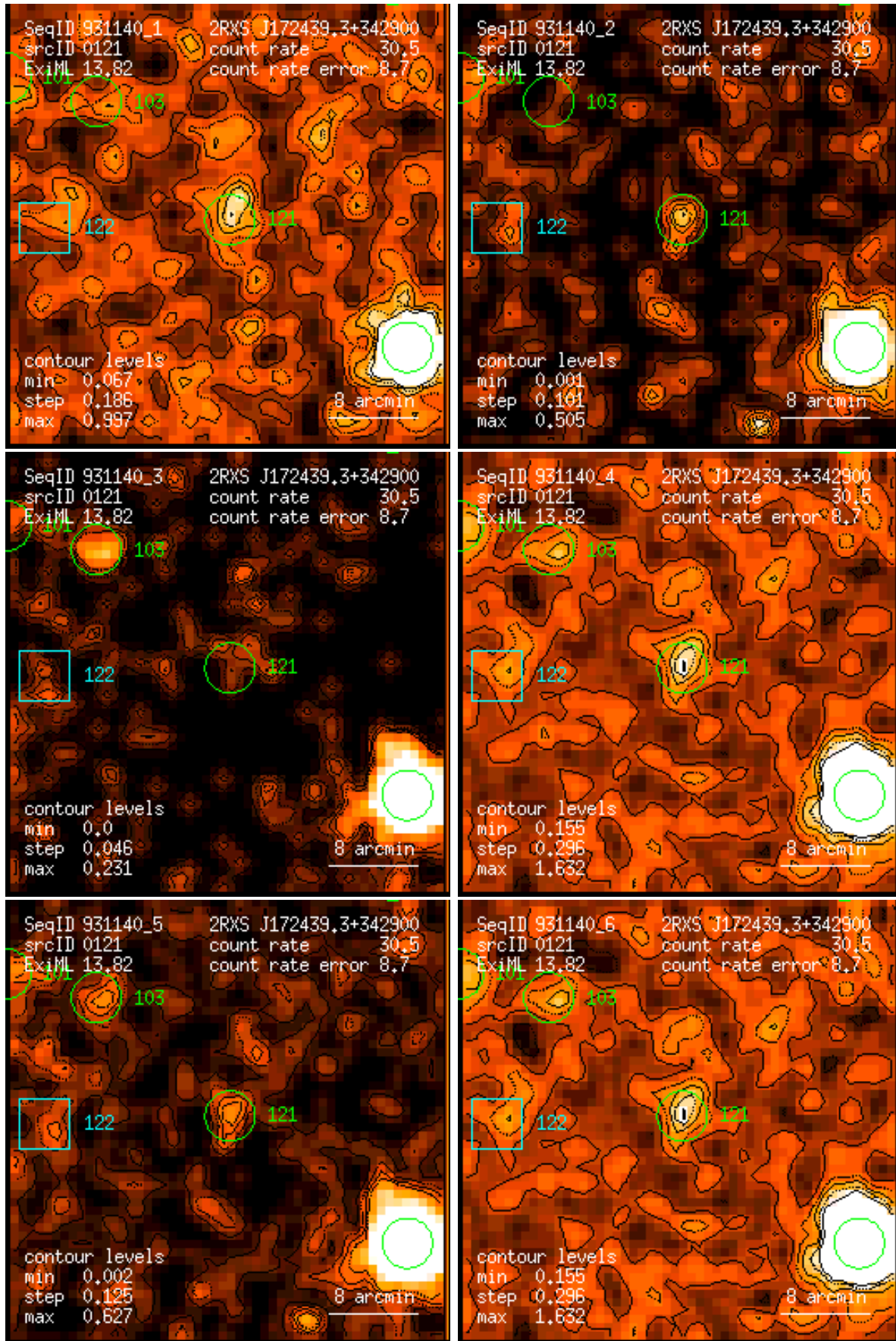
Figure 121: RASS 931140: detection 0121: band rate images, Gaussian filter: (1) PSPC channels 11 – 41, (2) 52 – 90, (3) 91 – 201, (4) 11 – 235, (5) 52 – 201, (6) 11 – 201. Broad band rates in counts/ks. Band rate contour levels in counts/ks/arcmin 2 .
