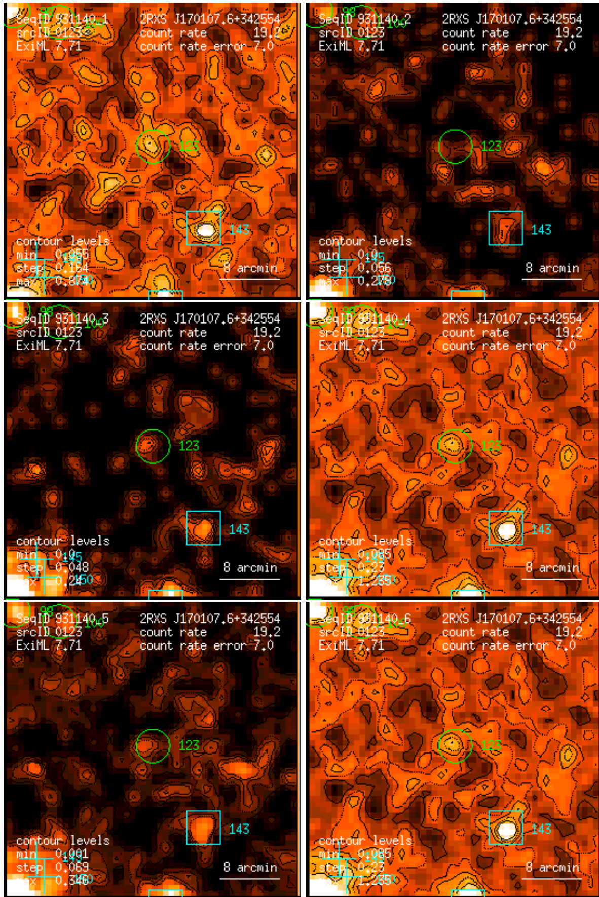
Figure 123: RASS 931140: detection 0123: band rate images, Gaussian filter: (1) PSPC channels 11 – 41, (2) 52 – 90, (3) 91 – 201, (4) 11 – 235, (5) 52 – 201, (6) 11 – 201. Broad band rates in counts/ks. Band rate contour levels in counts/ks/arcmin 2 .
