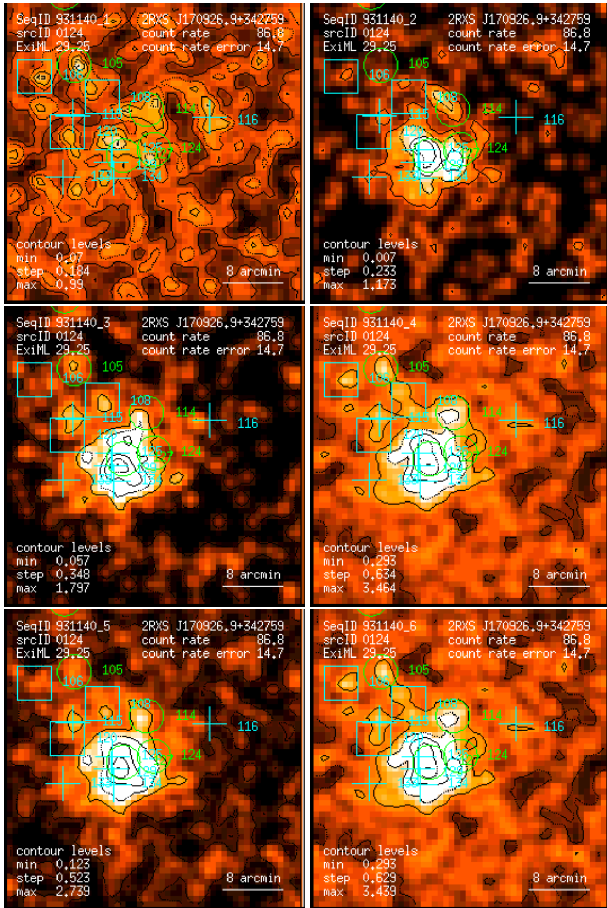
Figure 124: RASS 931140: detection 0124: band rate images, Gaussian filter: (1) PSPC channels 11 – 41, (2) 52 – 90, (3) 91 – 201, (4) 11 – 235, (5) 52 – 201, (6) 11 – 201. Broad band rates in counts/ks. Band rate contour levels in counts/ks/arcmin 2 .
