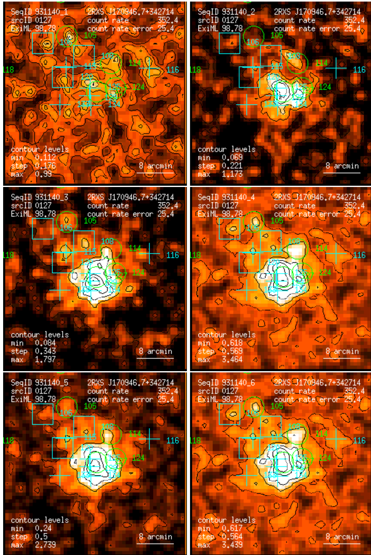
Figure 127: RASS 931140: detection 0127: band rate images, Gaussian filter: (1) PSPC channels 11 – 41, (2) 52 – 90, (3) 91 – 201, (4) 11 – 235, (5) 52 – 201, (6) 11 – 201. Broad band rates in counts/ks. Band rate contour levels in counts/ks/arcmin 2 .
