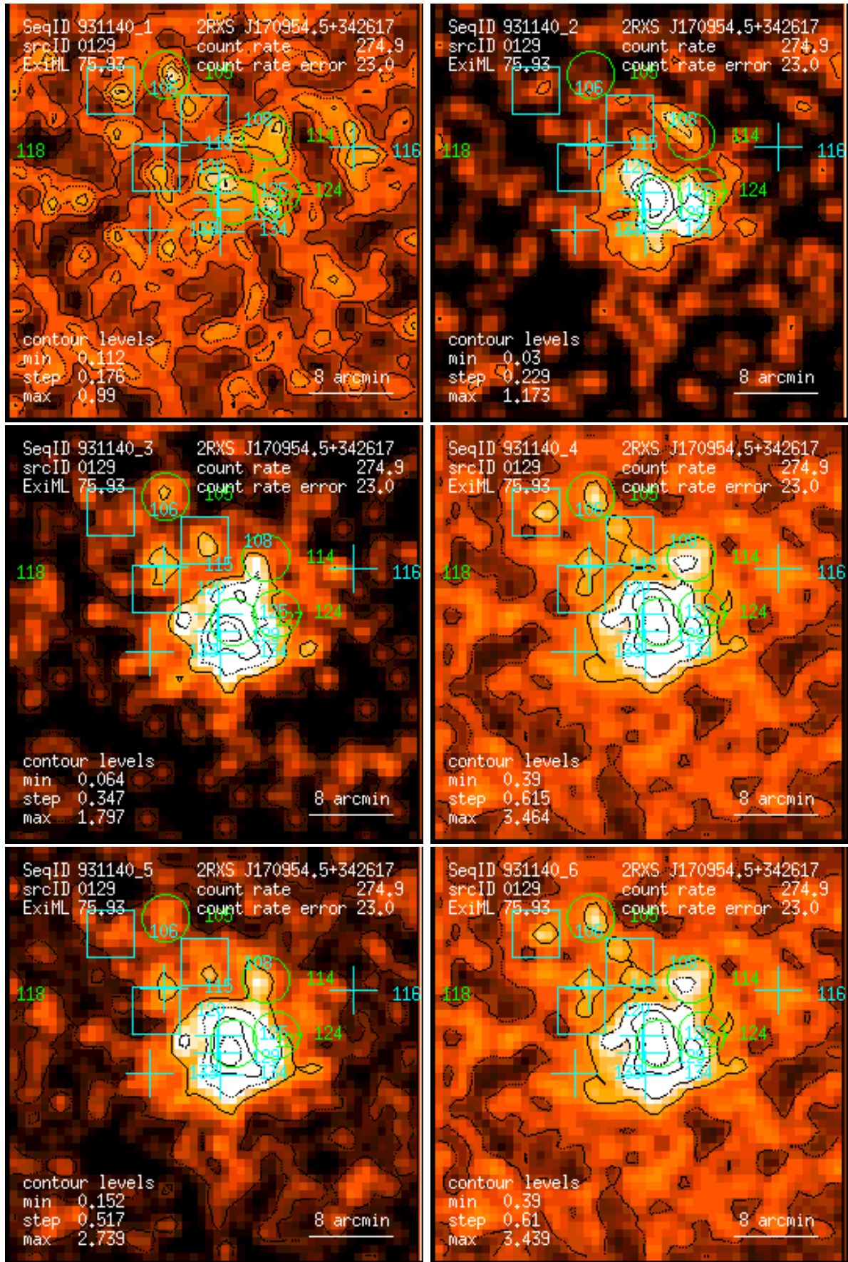
Figure 129: RASS 931140: detection 0129: band rate images, Gaussian filter: (1) PSPC channels 11 – 41, (2) 52 – 90, (3) 91 – 201, (4) 11 – 235, (5) 52 – 201, (6) 11 – 201. Broad band rates in counts/ks. Band rate contour levels in counts/ks/arcmin 2 .
