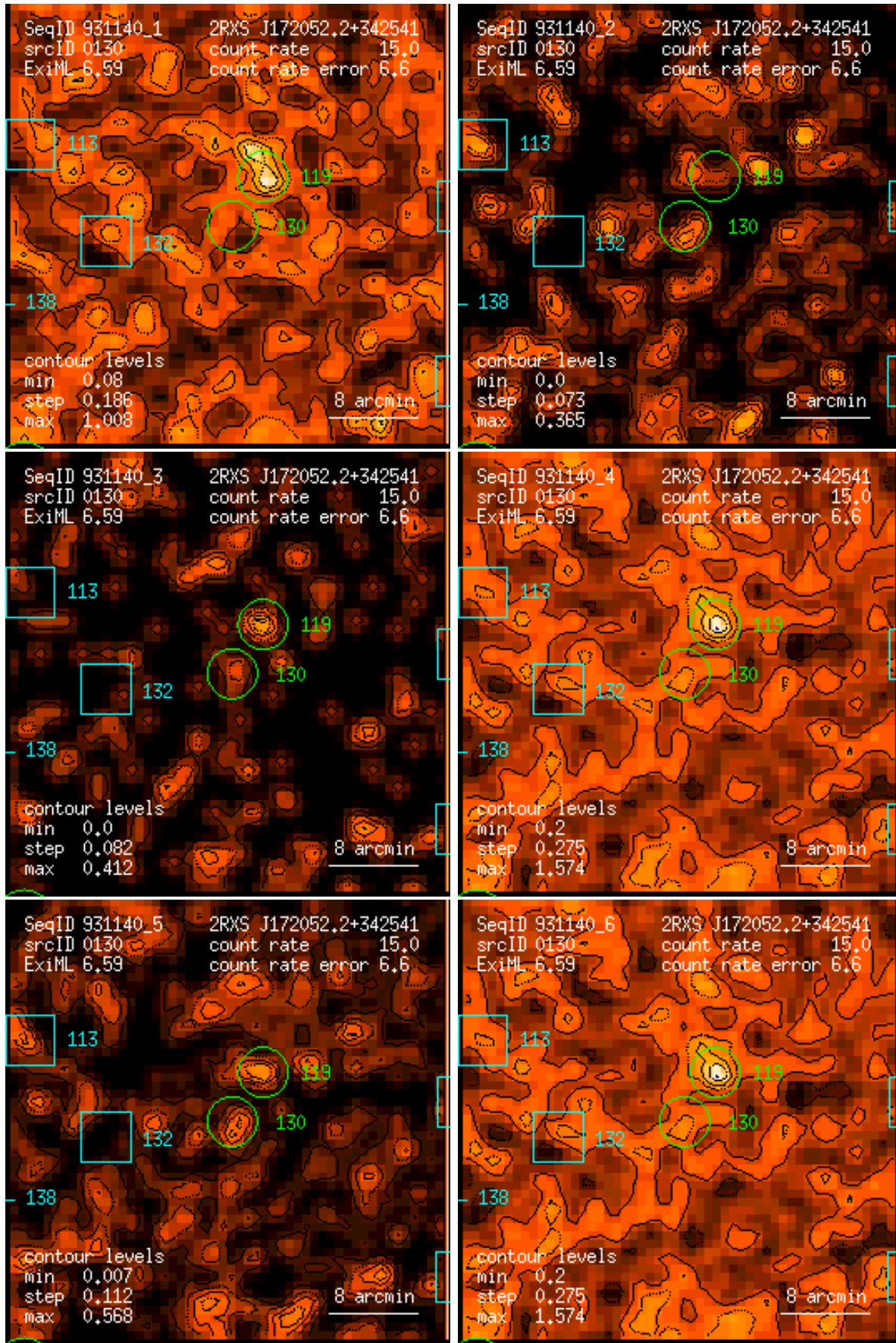
Figure 130: RASS 931140: detection 0130: band rate images, Gaussian filter: (1) PSPC channels 11 – 41, (2) 52 – 90, (3) 91 – 201, (4) 11 – 235, (5) 52 – 201, (6) 11 – 201. Broad band rates in counts/ks. Band rate contour levels in counts/ks/arcmin 2 .
