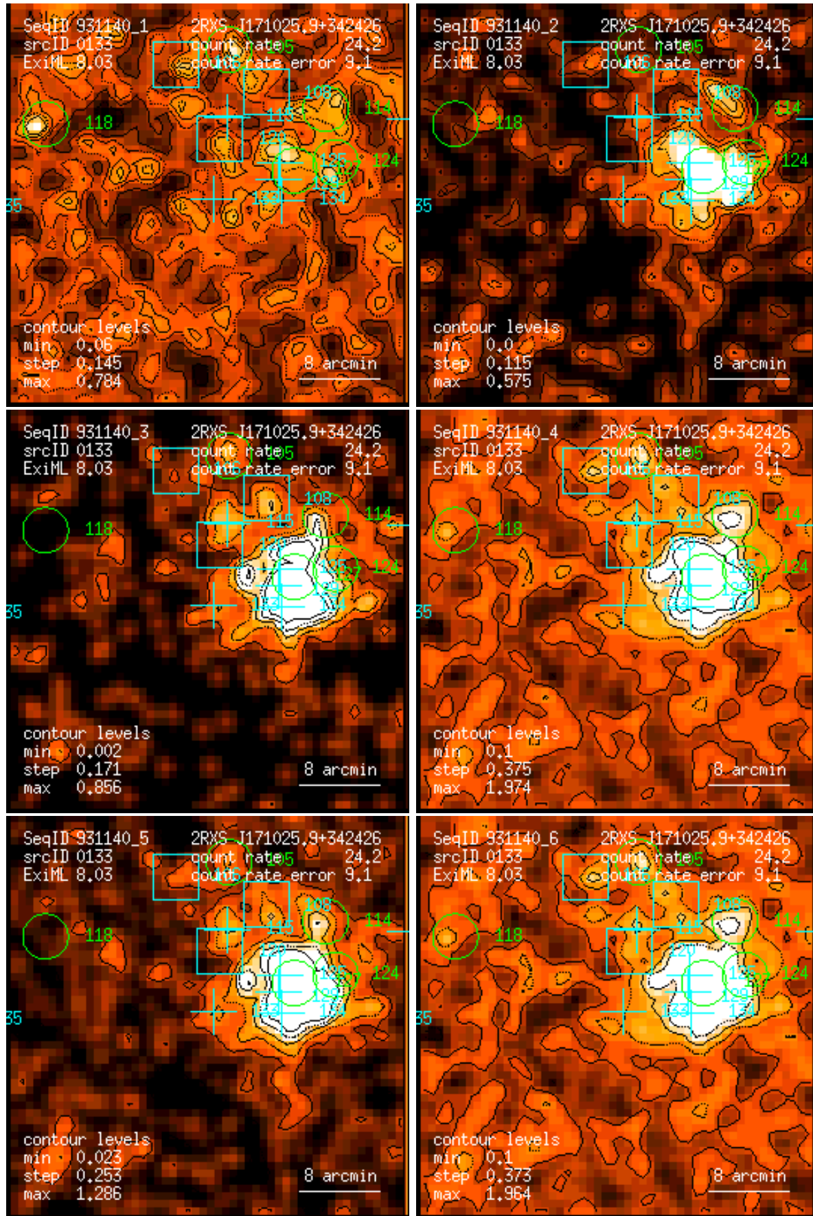
Figure 133: RASS 931140: detection 0133: band rate images, Gaussian filter: (1) PSPC channels 11 – 41, (2) 52 – 90, (3) 91 – 201, (4) 11 – 235, (5) 52 – 201, (6) 11 – 201. Broad band rates in counts/ks. Band rate contour levels in counts/ks/arcmin 2 .
