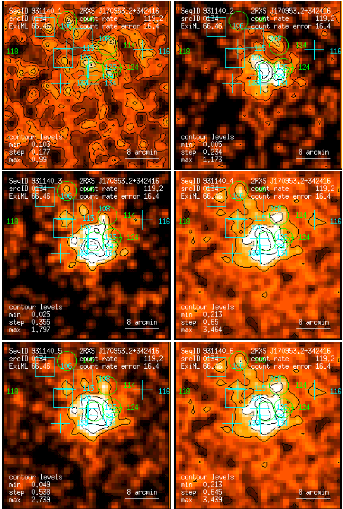
Figure 134: RASS 931140: detection 0134: band rate images, Gaussian filter: (1) PSPC channels 11 – 41, (2) 52 – 90, (3) 91 – 201, (4) 11 – 235, (5) 52 – 201, (6) 11 – 201. Broad band rates in counts/ks. Band rate contour levels in counts/ks/arcmin 2 .
