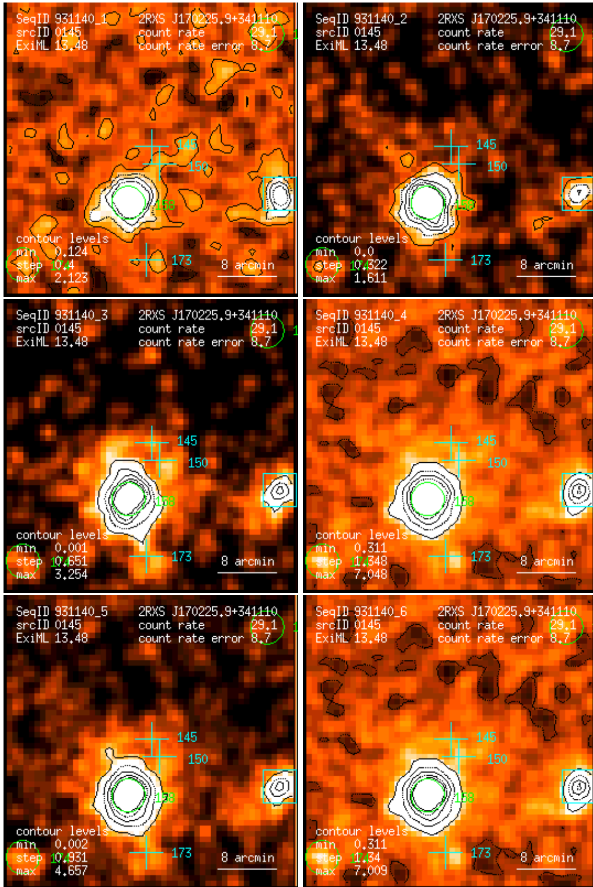
Figure 145: RASS 931140: detection 0145: band rate images, Gaussian filter: (1) PSPC channels 11 – 41, (2) 52 – 90, (3) 91 – 201, (4) 11 – 235, (5) 52 – 201, (6) 11 – 201. Broad band rates in counts/ks. Band rate contour levels in counts/ks/arcmin 2 .
