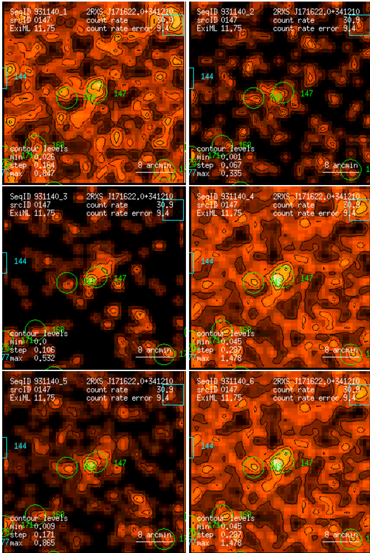
Figure 147: RASS 931140: detection 0147: band rate images, Gaussian filter: (1) PSPC channels 11 – 41, (2) 52 – 90, (3) 91 – 201, (4) 11 – 235, (5) 52 – 201, (6) 11 – 201. Broad band rates in counts/ks. Band rate contour levels in counts/ks/arcmin 2 .
