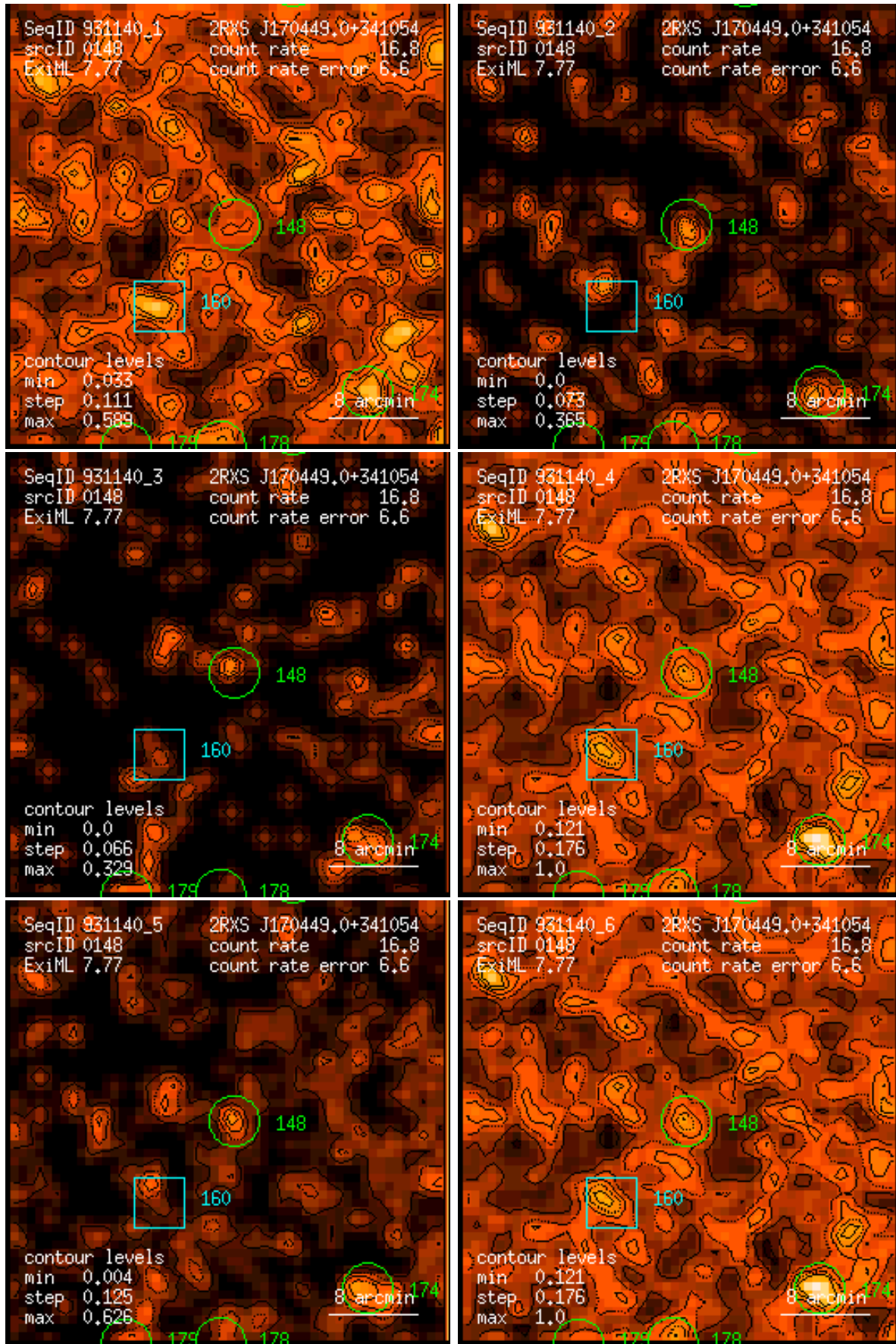
Figure 148: RASS 931140: detection 0148: band rate images, Gaussian filter: (1) PSPC channels 11 – 41, (2) 52 – 90, (3) 91 – 201, (4) 11 – 235, (5) 52 – 201, (6) 11 – 201. Broad band rates in counts/ks. Band rate contour levels in counts/ks/arcmin 2 .
