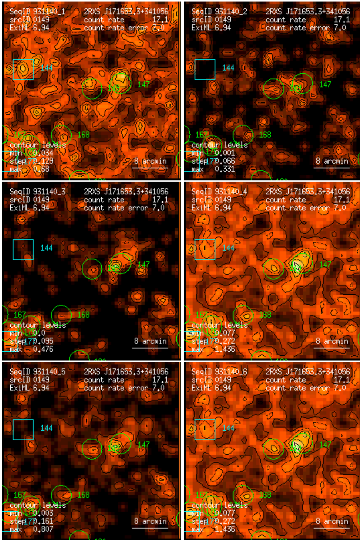
Figure 149: RASS 931140: detection 0149: band rate images, Gaussian filter: (1) PSPC channels 11 – 41, (2) 52 – 90, (3) 91 – 201, (4) 11 – 235, (5) 52 – 201, (6) 11 – 201. Broad band rates in counts/ks. Band rate contour levels in counts/ks/arcmin 2 .
