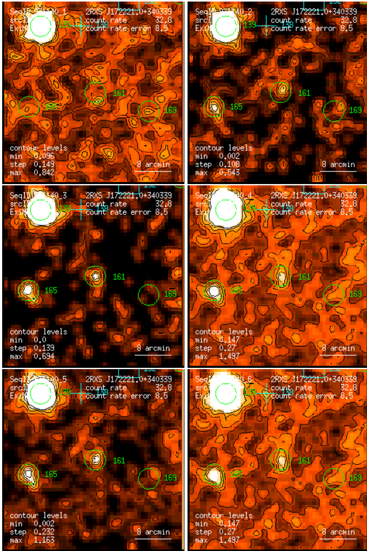
Figure 161: RASS 931140: detection 0161: band rate images, Gaussian filter: (1) PSPC channels 11 – 41, (2) 52 – 90, (3) 91 – 201, (4) 11 – 235, (5) 52 – 201, (6) 11 – 201. Broad band rates in counts/ks. Band rate contour levels in counts/ks/arcmin 2 .
