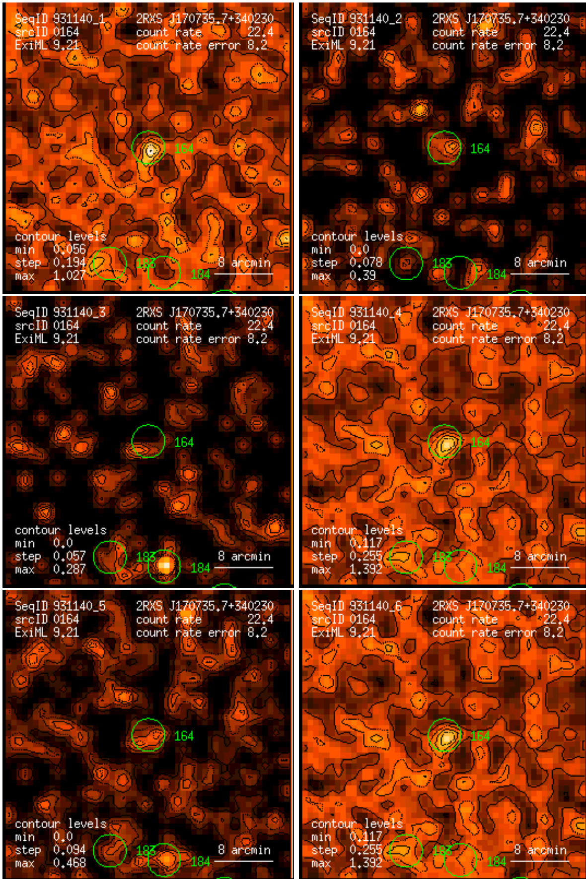
Figure 164: RASS 931140: detection 0164: band rate images, Gaussian filter: (1) PSPC channels 11 – 41, (2) 52 – 90, (3) 91 – 201, (4) 11 – 235, (5) 52 – 201, (6) 11 – 201. Broad band rates in counts/ks. Band rate contour levels in counts/ks/arcmin 2 .
