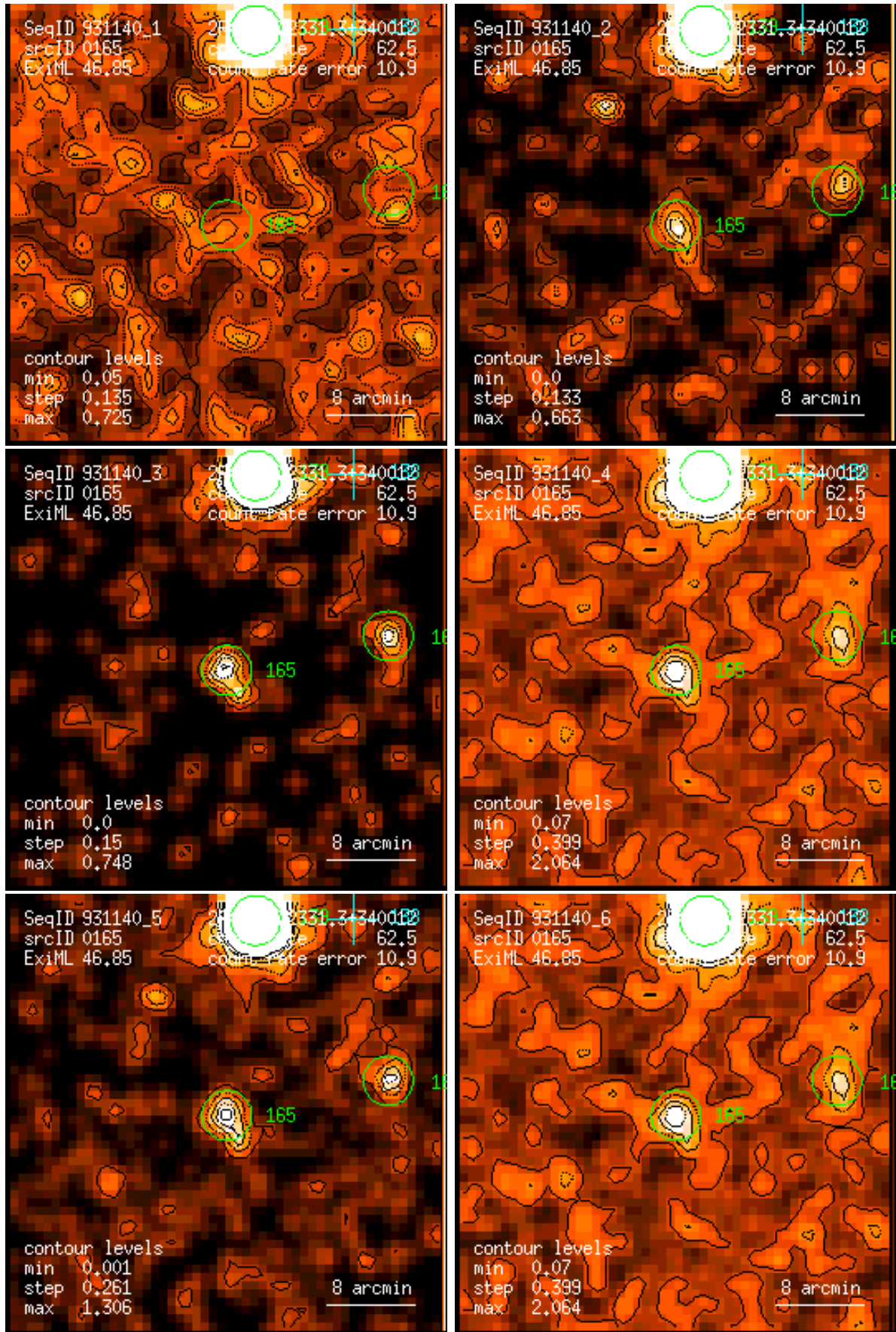
Figure 165: RASS 931140: detection 0165: band rate images, Gaussian filter: (1) PSPC channels 11 – 41, (2) 52 – 90, (3) 91 – 201, (4) 11 – 235, (5) 52 – 201, (6) 11 – 201. Broad band rates in counts/ks. Band rate contour levels in counts/ks/arcmin 2 .
