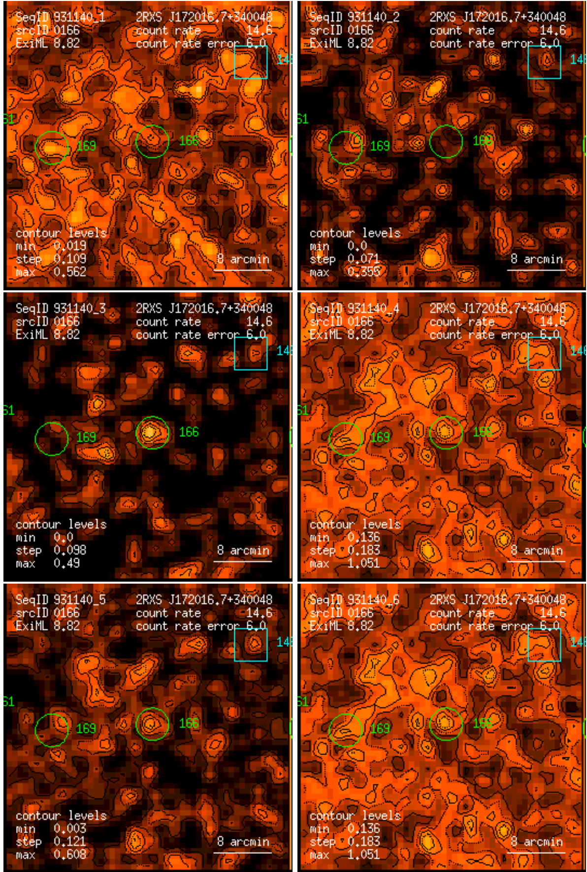
Figure 166: RASS 931140: detection 0166: band rate images, Gaussian filter: (1) PSPC channels 11 – 41, (2) 52 – 90, (3) 91 – 201, (4) 11 – 235, (5) 52 – 201, (6) 11 – 201. Broad band rates in counts/ks. Band rate contour levels in counts/ks/arcmin 2 .
