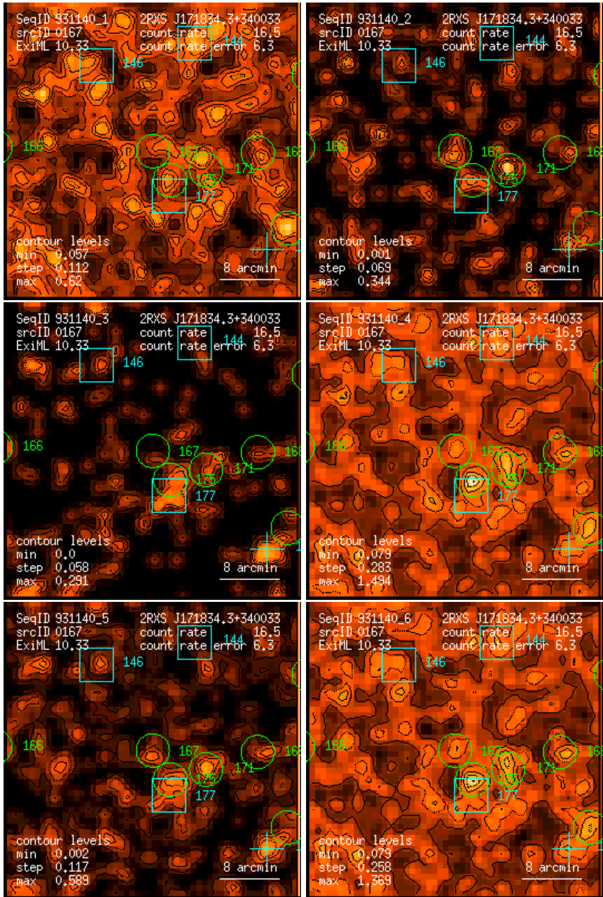
Figure 167: RASS 931140: detection 0167: band rate images, Gaussian filter: (1) PSPC channels 11 – 41, (2) 52 – 90, (3) 91 – 201, (4) 11 – 235, (5) 52 – 201, (6) 11 – 201. Broad band rates in counts/ks. Band rate contour levels in counts/ks/arcmin 2 .
