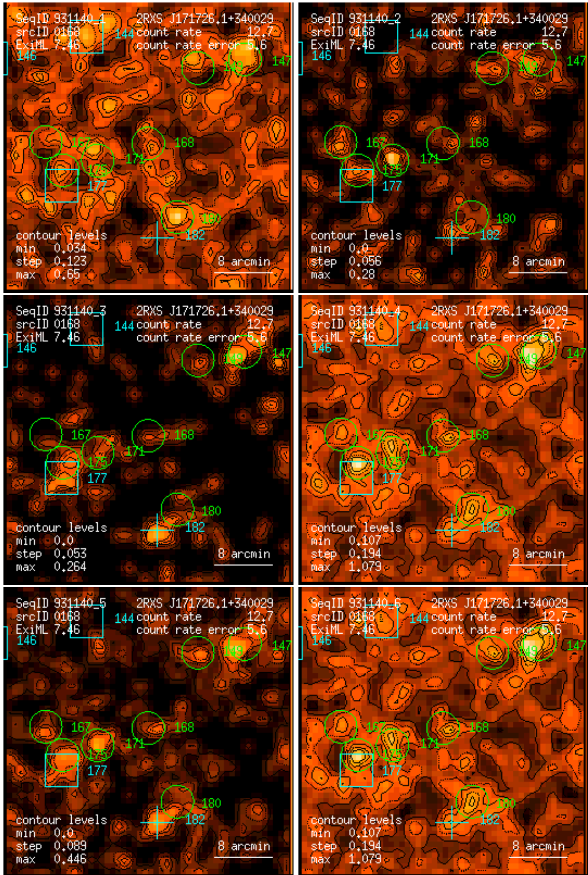
Figure 168: RASS 931140: detection 0168: band rate images, Gaussian filter: (1) PSPC channels 11 – 41, (2) 52 – 90, (3) 91 – 201, (4) 11 – 235, (5) 52 – 201, (6) 11 – 201. Broad band rates in counts/ks. Band rate contour levels in counts/ks/arcmin 2 .
