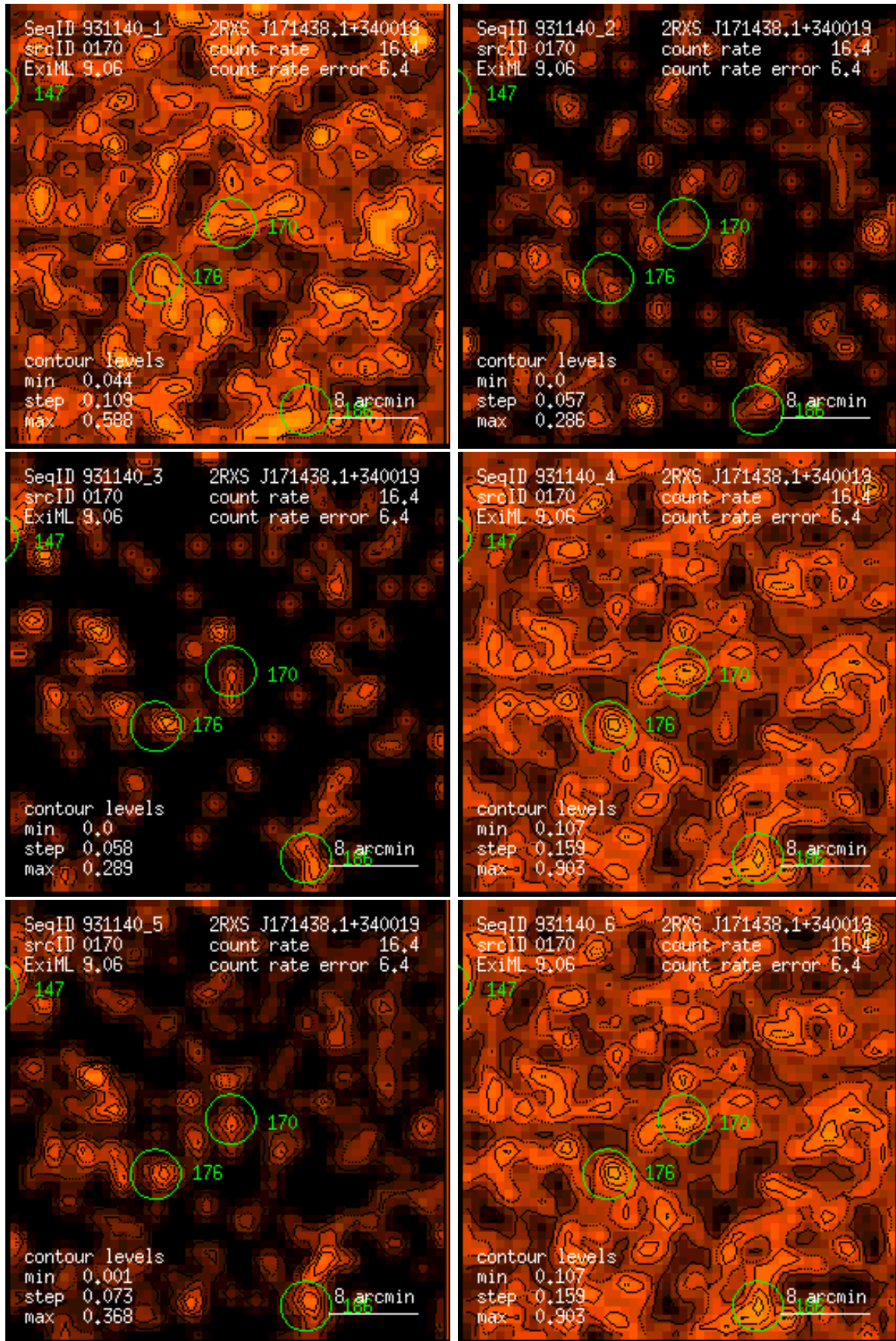
Figure 170: RASS 931140: detection 0170: band rate images, Gaussian filter: (1) PSPC channels 11 – 41, (2) 52 – 90, (3) 91 – 201, (4) 11 – 235, (5) 52 – 201, (6) 11 – 201. Broad band rates in counts/ks. Band rate contour levels in counts/ks/arcmin 2 .
